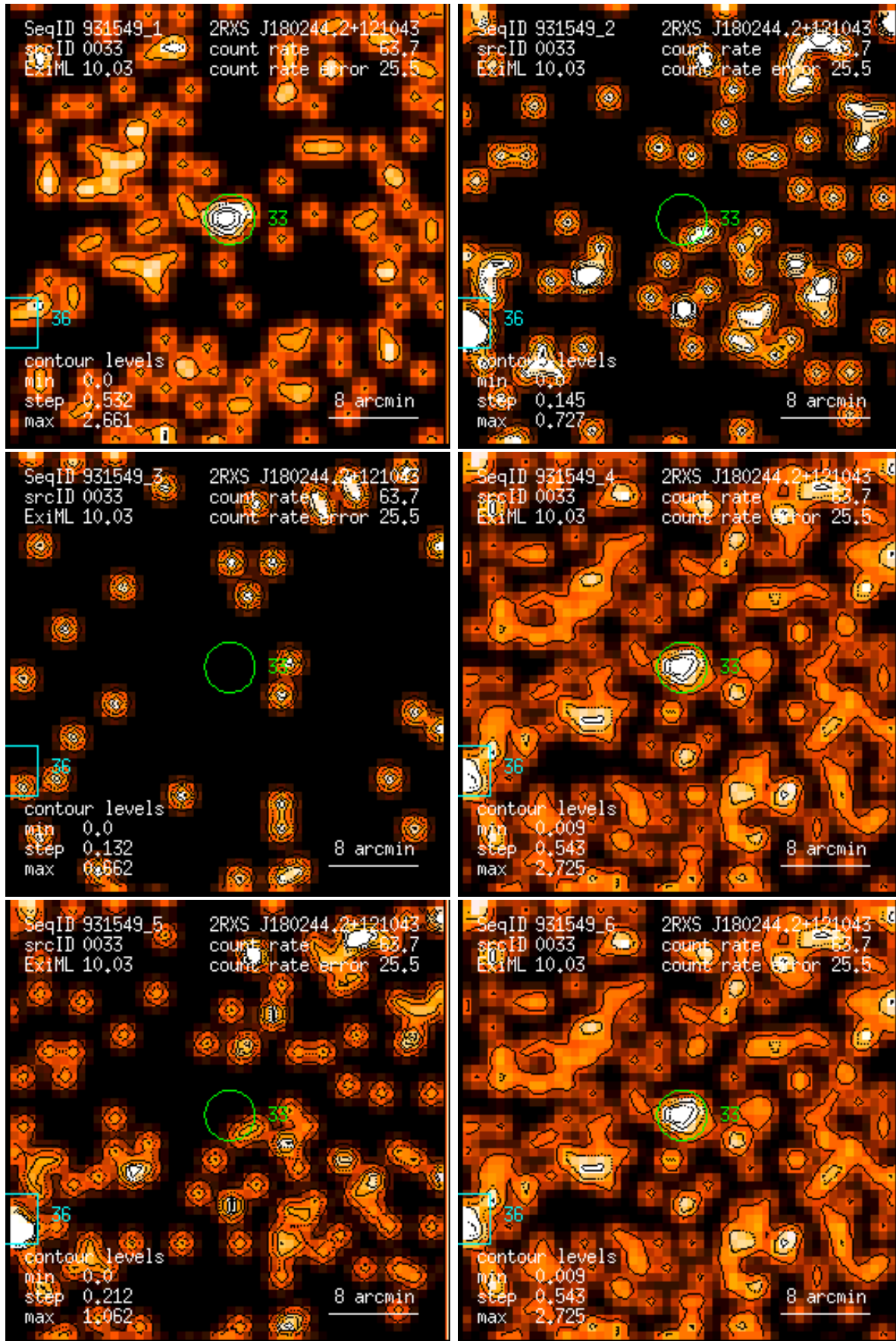
Figure 33: RASS 931549: detection 0033: band rate images, Gaussian filter: (1) PSPC channels 11 – 41, (2) 52 – 90, (3) 91 – 201, (4) 11 – 235, (5) 52 – 201, (6) 11 – 201. Broad band rates in counts/ks. Band rate contour levels in counts/ks/arcmin 2 .
