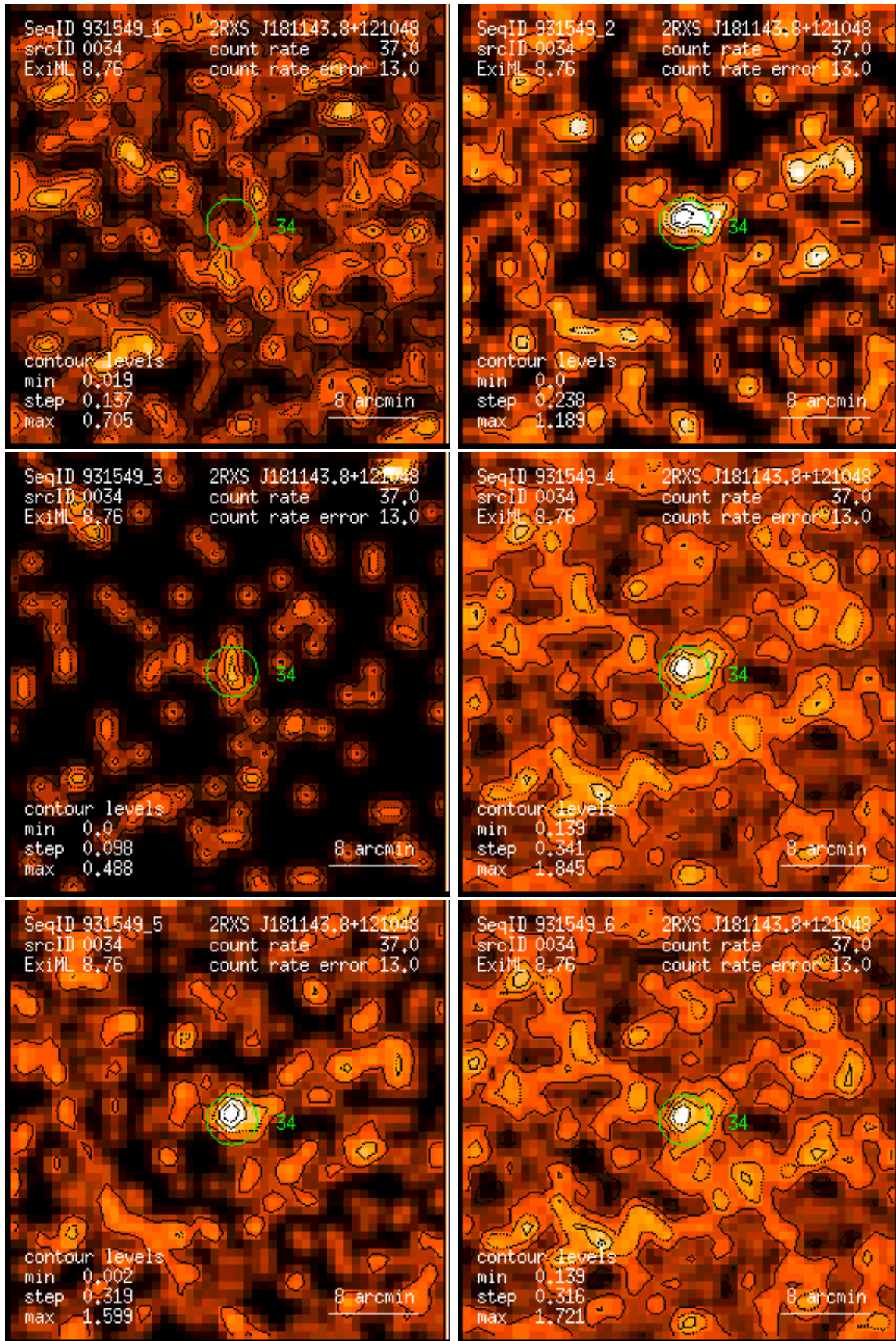
Figure 34: RASS 931549: detection 0034: band rate images, Gaussian filter: (1) PSPC channels 11 – 41, (2) 52 – 90, (3) 91 – 201, (4) 11 – 235, (5) 52 – 201, (6) 11 – 201. Broad band rates in counts/ks. Band rate contour levels in counts/ks/arcmin 2 .
