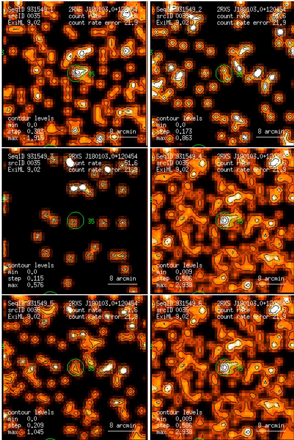
Figure 35: RASS 931549: detection 0035: band rate images, Gaussian filter: (1) PSPC channels 11 – 41, (2) 52 – 90, (3) 91 – 201, (4) 11 – 235, (5) 52 – 201, (6) 11 – 201. Broad band rates in counts/ks. Band rate contour levels in counts/ks/arcmin 2 .
