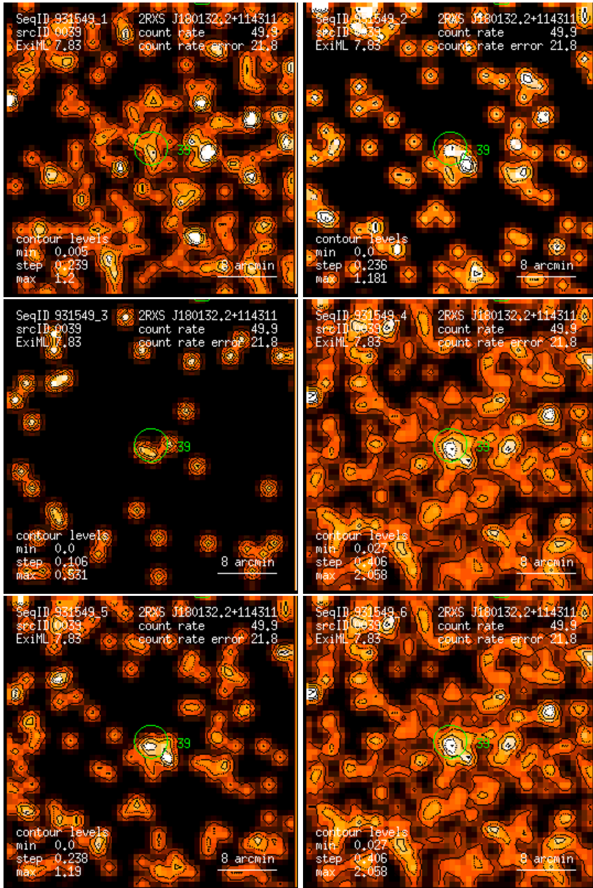
Figure 39: RASS 931549: detection 0039: band rate images, Gaussian filter: (1) PSPC channels 11 – 41, (2) 52 – 90, (3) 91 – 201, (4) 11 – 235, (5) 52 – 201, (6) 11 – 201. Broad band rates in counts/ks. Band rate contour levels in counts/ks/arcmin 2 .
