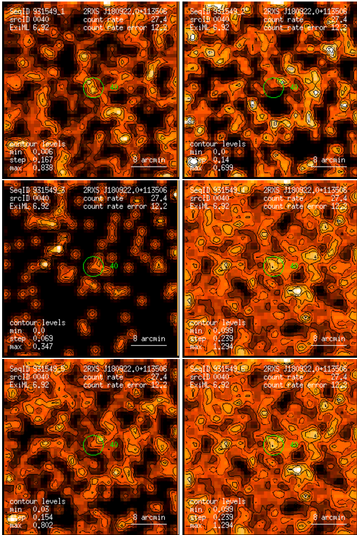
Figure 40: RASS 931549: detection 0040: band rate images, Gaussian filter: (1) PSPC channels 11 – 41, (2) 52 – 90, (3) 91 – 201, (4) 11 – 235, (5) 52 – 201, (6) 11 – 201. Broad band rates in counts/ks. Band rate contour levels in counts/ks/arcmin 2 .
