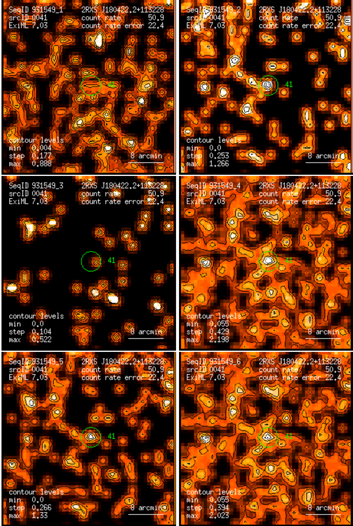
Figure 41: RASS 931549: detection 0041: band rate images, Gaussian filter: (1) PSPC channels 11 – 41, (2) 52 – 90, (3) 91 – 201, (4) 11 – 235, (5) 52 – 201, (6) 11 – 201. Broad band rates in counts/ks. Band rate contour levels in counts/ks/arcmin 2 .
