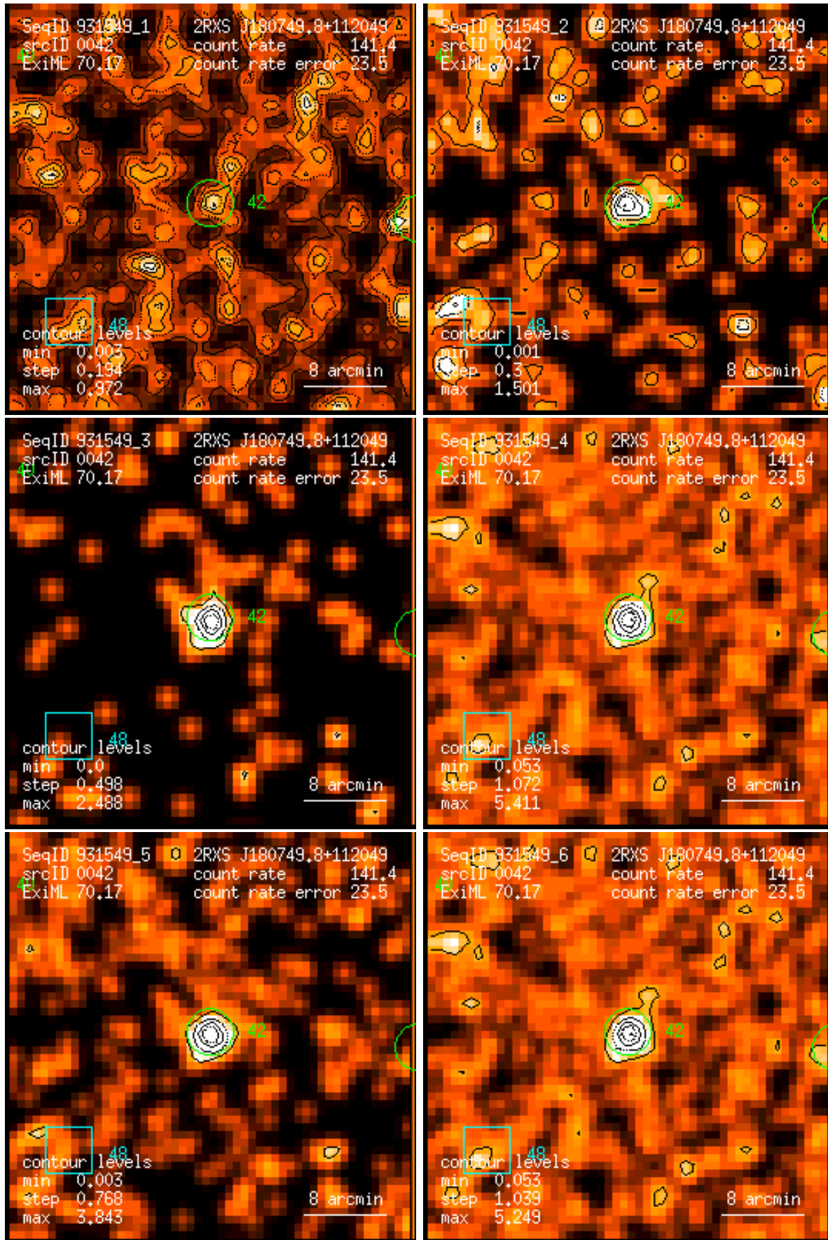
Figure 42: RASS 931549: detection 0042: band rate images, Gaussian filter: (1) PSPC channels 11 – 41, (2) 52 – 90, (3) 91 – 201, (4) 11 – 235, (5) 52 – 201, (6) 11 – 201. Broad band rates in counts/ks. Band rate contour levels in counts/ks/arcmin 2 .
