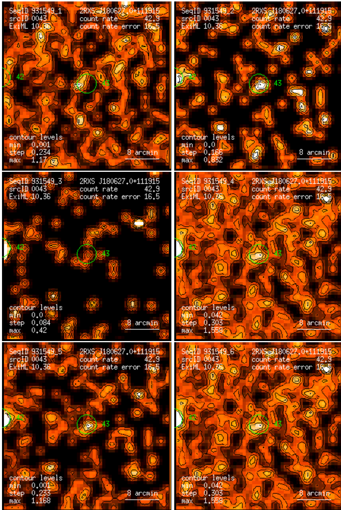
Figure 43: RASS 931549: detection 0043: band rate images, Gaussian filter: (1) PSPC channels 11 – 41, (2) 52 – 90, (3) 91 – 201, (4) 11 – 235, (5) 52 – 201, (6) 11 – 201. Broad band rates in counts/ks. Band rate contour levels in counts/ks/arcmin 2 .
