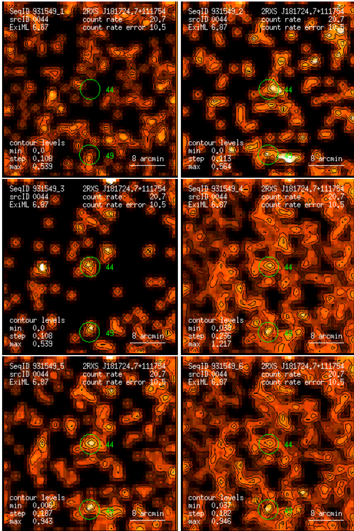
Figure 44: RASS 931549: detection 0044: band rate images, Gaussian filter: (1) PSPC channels 11 – 41, (2) 52 – 90, (3) 91 – 201, (4) 11 – 235, (5) 52 – 201, (6) 11 – 201. Broad band rates in counts/ks. Band rate contour levels in counts/ks/arcmin 2 .
