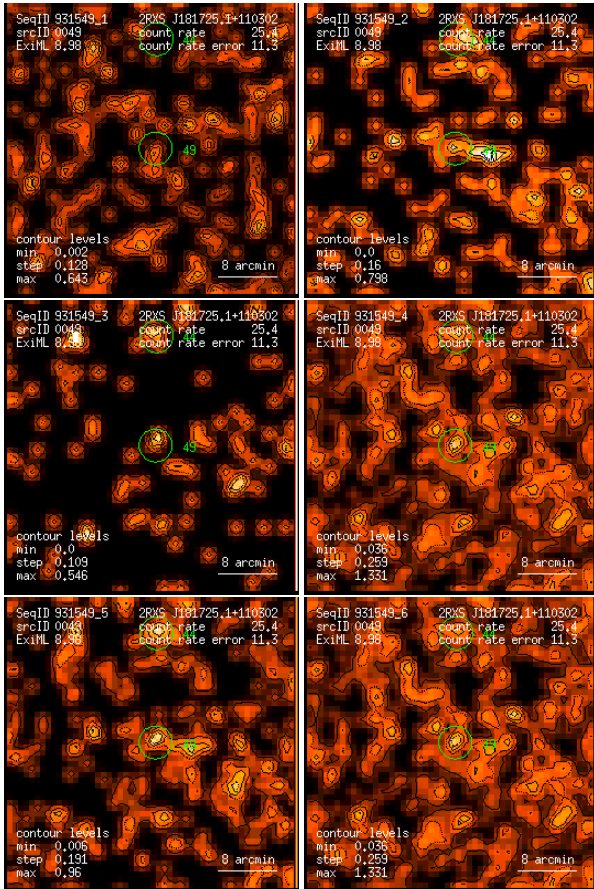
Figure 49: RASS 931549: detection 0049: band rate images, Gaussian filter: (1) PSPC channels 11 – 41, (2) 52 – 90, (3) 91 – 201, (4) 11 – 235, (5) 52 – 201, (6) 11 – 201. Broad band rates in counts/ks. Band rate contour levels in counts/ks/arcmin 2 .
