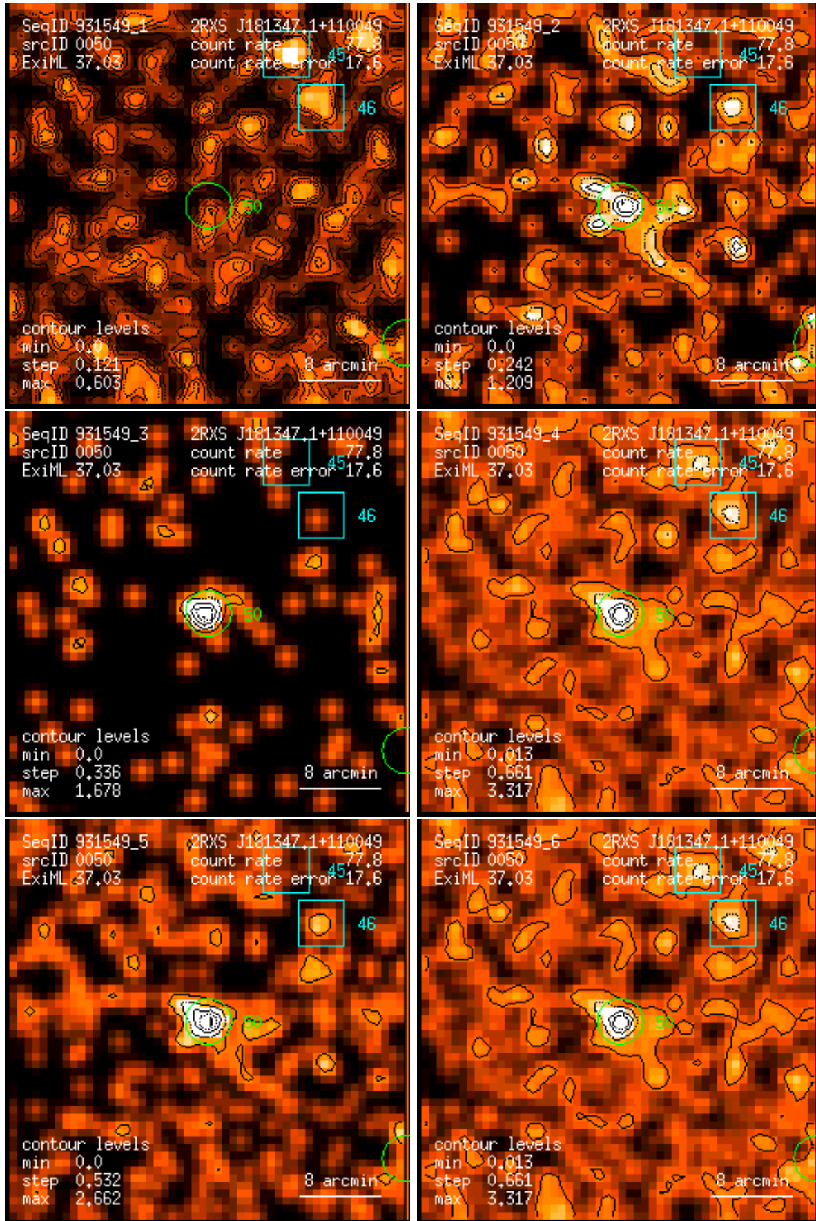
Figure 50: RASS 931549: detection 0050: band rate images, Gaussian filter: (1) PSPC channels 11 – 41, (2) 52 – 90, (3) 91 – 201, (4) 11 – 235, (5) 52 – 201, (6) 11 – 201. Broad band rates in counts/ks. Band rate contour levels in counts/ks/arcmin 2 .
