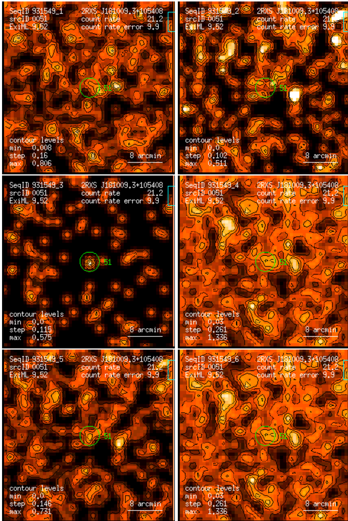
Figure 51: RASS 931549: detection 0051: band rate images, Gaussian filter: (1) PSPC channels 11 – 41, (2) 52 – 90, (3) 91 – 201, (4) 11 – 235, (5) 52 – 201, (6) 11 – 201. Broad band rates in counts/ks. Band rate contour levels in counts/ks/arcmin 2 .
