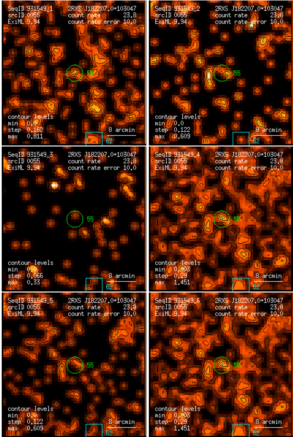
Figure 55: RASS 931549: detection 0055: band rate images, Gaussian filter: (1) PSPC channels 11 – 41, (2) 52 – 90, (3) 91 – 201, (4) 11 – 235, (5) 52 – 201, (6) 11 – 201. Broad band rates in counts/ks. Band rate contour levels in counts/ks/arcmin 2 .
