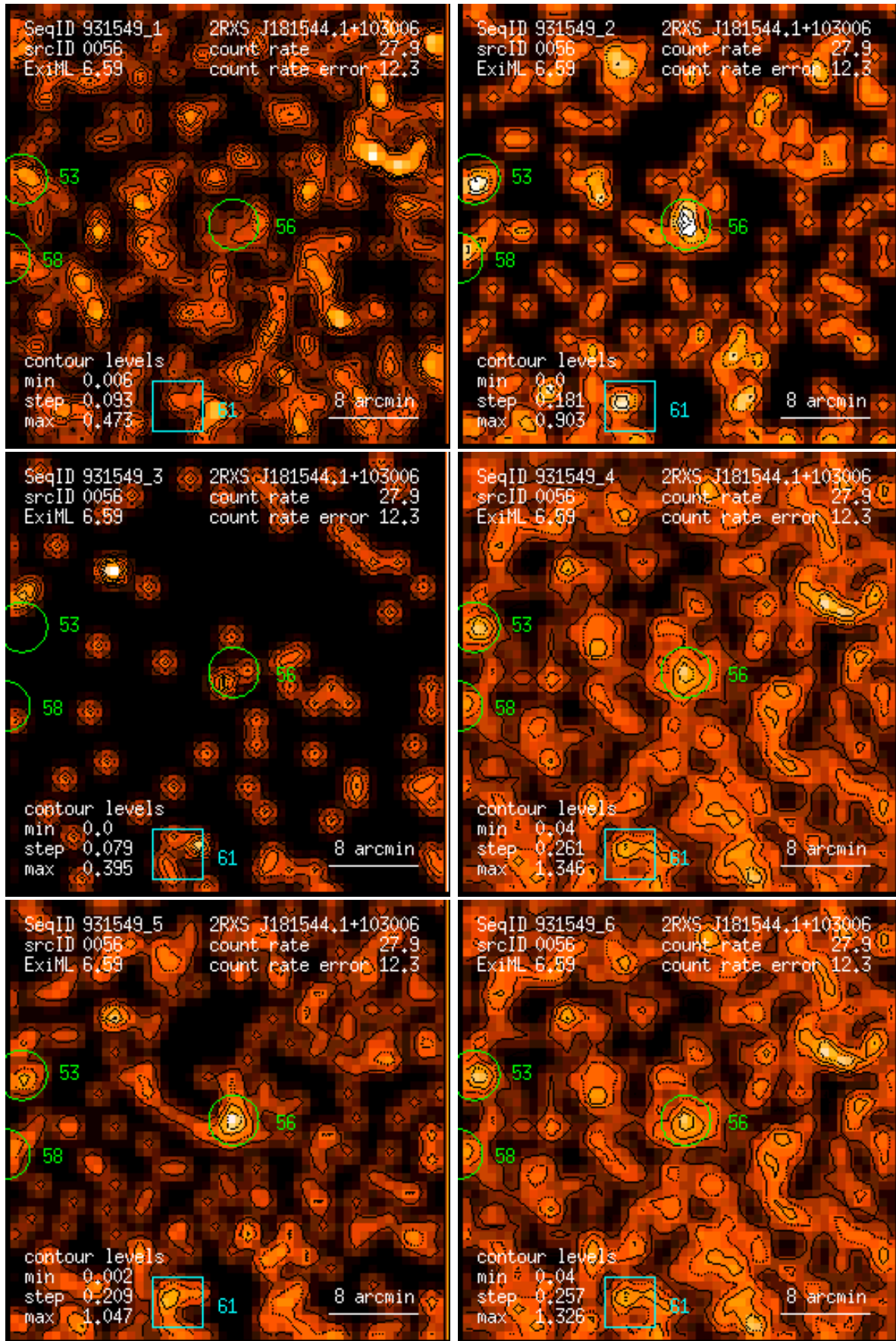
Figure 56: RASS 931549: detection 0056: band rate images, Gaussian filter: (1) PSPC channels 11 – 41, (2) 52 – 90, (3) 91 – 201, (4) 11 – 235, (5) 52 – 201, (6) 11 – 201. Broad band rates in counts/ks. Band rate contour levels in counts/ks/arcmin 2 .
