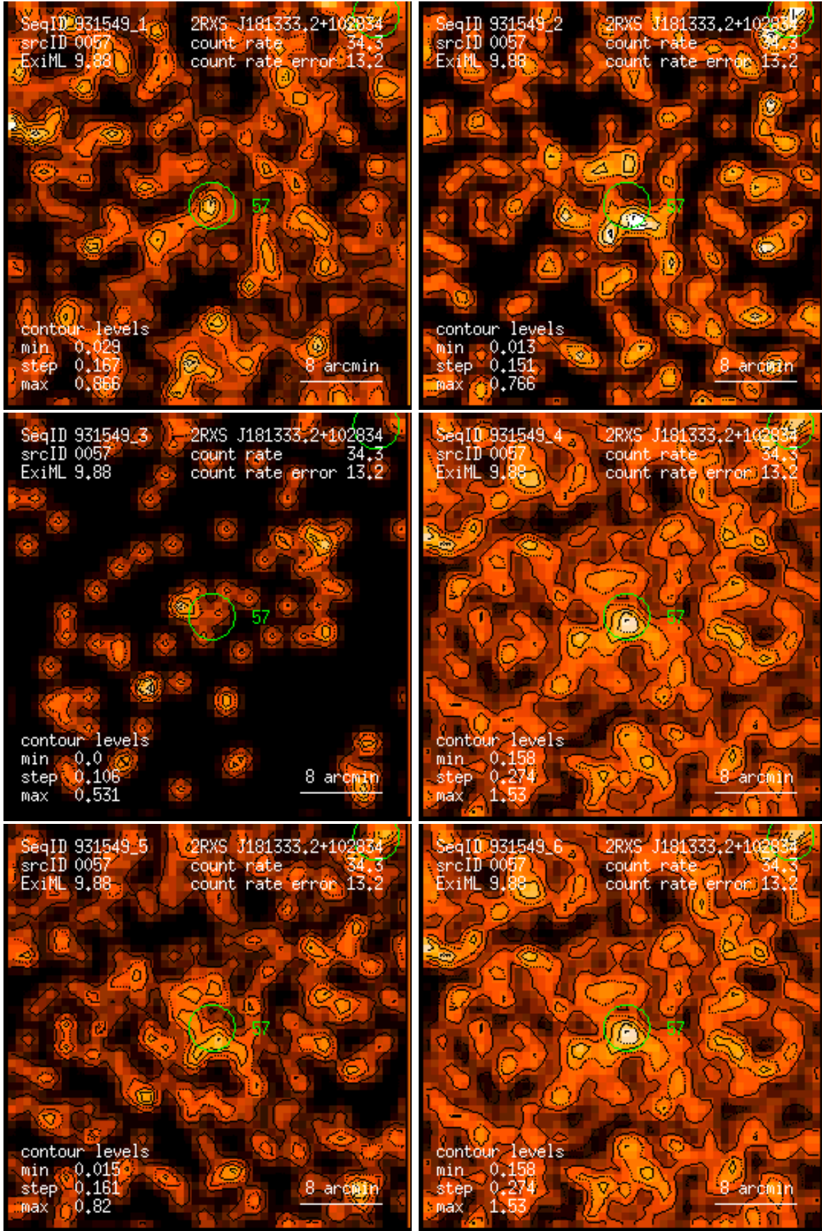
Figure 57: RASS 931549: detection 0057: band rate images, Gaussian filter: (1) PSPC channels 11 – 41, (2) 52 – 90, (3) 91 – 201, (4) 11 – 235, (5) 52 – 201, (6) 11 – 201. Broad band rates in counts/ks. Band rate contour levels in counts/ks/arcmin 2 .
