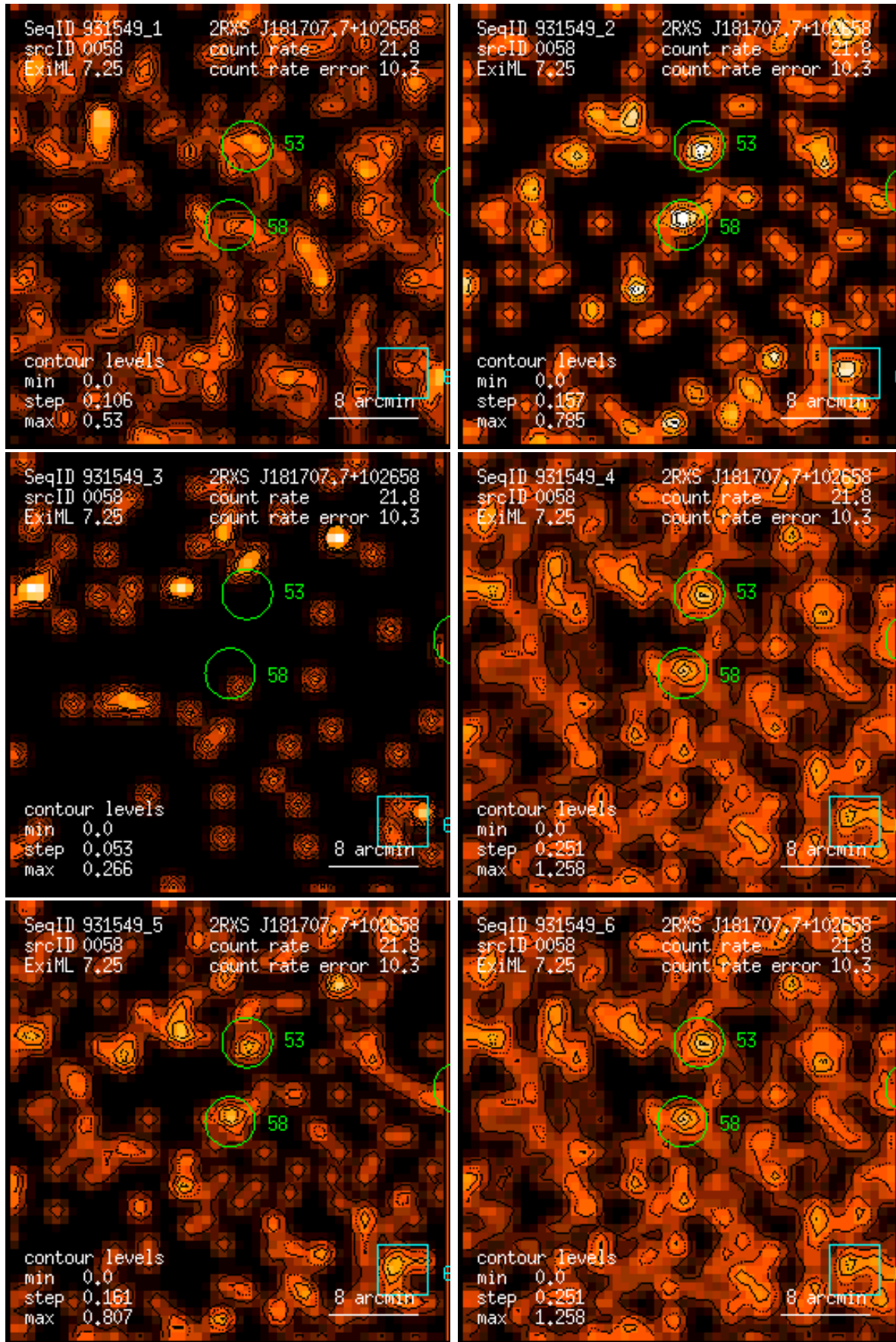
Figure 58: RASS 931549: detection 0058: band rate images, Gaussian filter: (1) PSPC channels 11 – 41, (2) 52 – 90, (3) 91 – 201, (4) 11 – 235, (5) 52 – 201, (6) 11 – 201. Broad band rates in counts/ks. Band rate contour levels in counts/ks/arcmin 2 .
