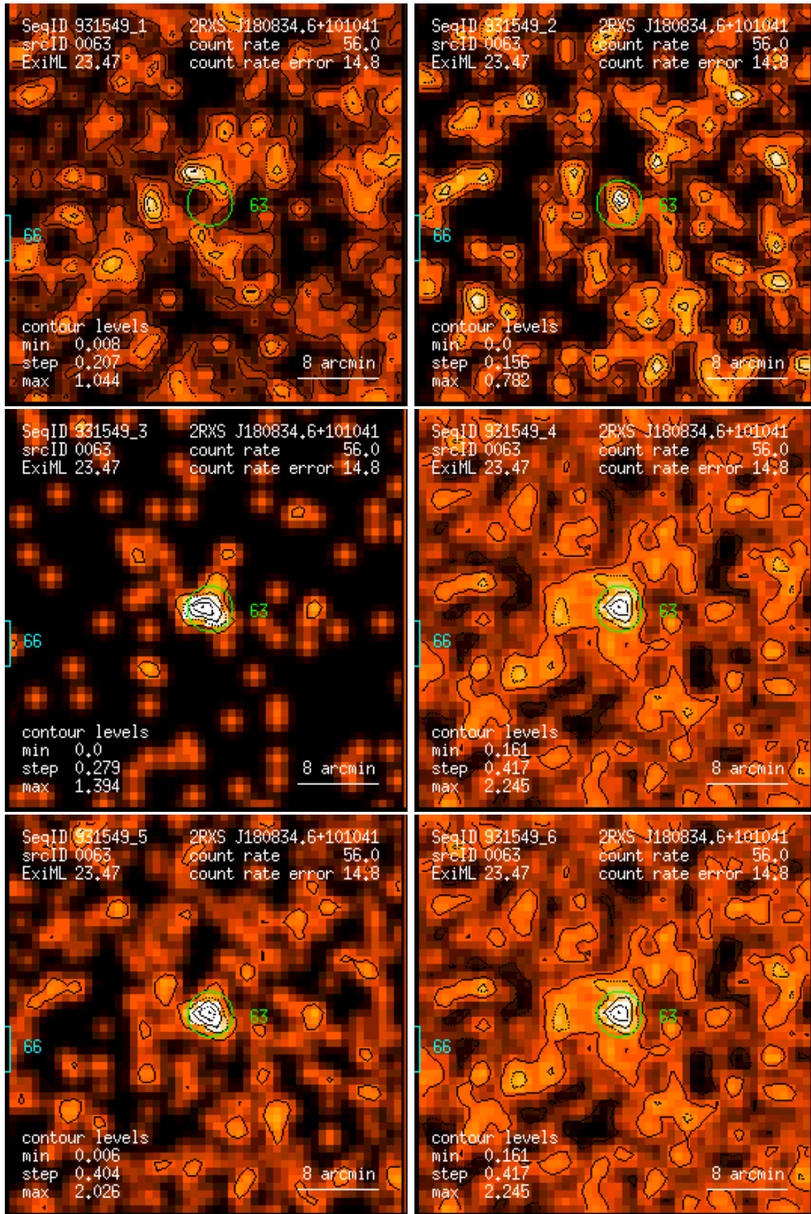
Figure 63: RASS 931549: detection 0063: band rate images, Gaussian filter: (1) PSPC channels 11 – 41, (2) 52 – 90, (3) 91 – 201, (4) 11 – 235, (5) 52 – 201, (6) 11 – 201. Broad band rates in counts/ks. Band rate contour levels in counts/ks/arcmin 2 .
