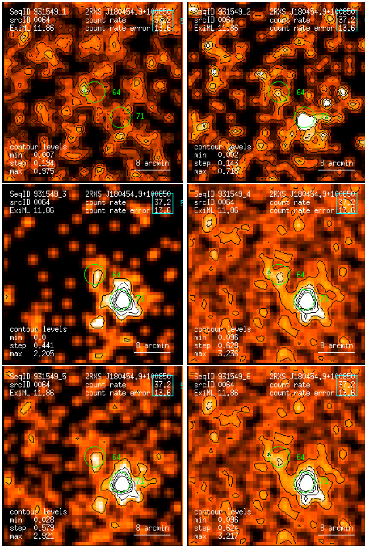
Figure 64: RASS 931549: detection 0064: band rate images, Gaussian filter: (1) PSPC channels 11 – 41, (2) 52 – 90, (3) 91 – 201, (4) 11 – 235, (5) 52 – 201, (6) 11 – 201. Broad band rates in counts/ks. Band rate contour levels in counts/ks/arcmin 2 .
