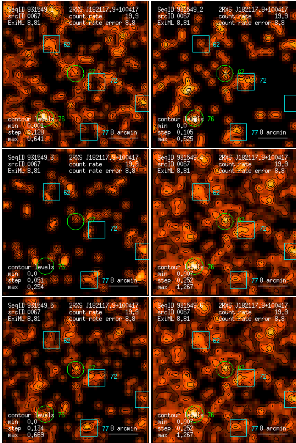
Figure 67: RASS 931549: detection 0067: band rate images, Gaussian filter: (1) PSPC channels 11 – 41, (2) 52 – 90, (3) 91 – 201, (4) 11 – 235, (5) 52 – 201, (6) 11 – 201. Broad band rates in counts/ks. Band rate contour levels in counts/ks/arcmin 2 .
