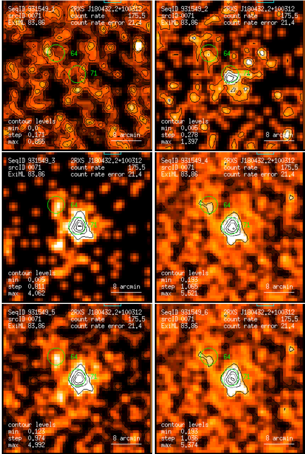
Figure 71: RASS 931549: detection 0071: band rate images, Gaussian filter: (1) PSPC channels 11 – 41, (2) 52 – 90, (3) 91 – 201, (4) 11 – 235, (5) 52 – 201, (6) 11 – 201. Broad band rates in counts/ks. Band rate contour levels in counts/ks/arcmin 2 .
