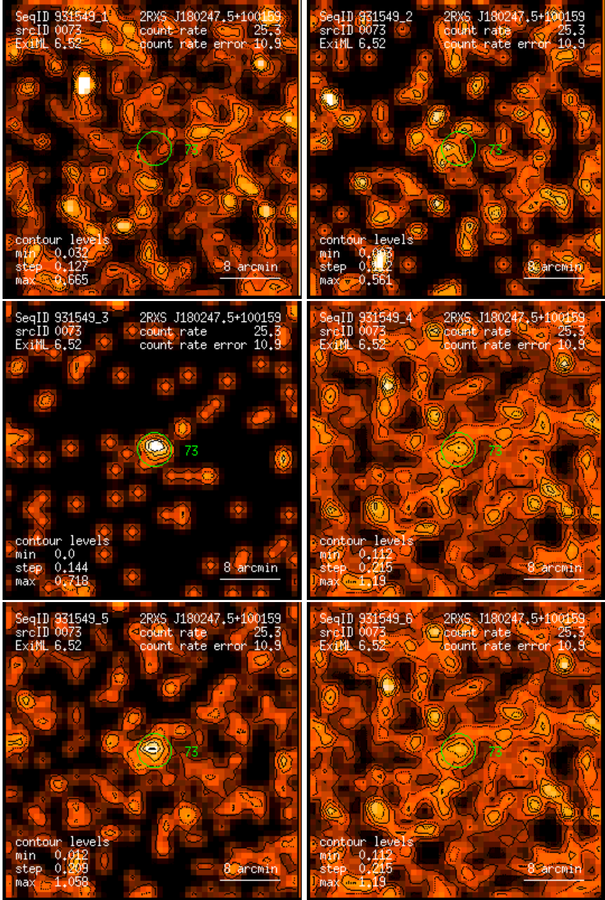
Figure 73: RASS 931549: detection 0073: band rate images, Gaussian filter: (1) PSPC channels 11 – 41, (2) 52 – 90, (3) 91 – 201, (4) 11 – 235, (5) 52 – 201, (6) 11 – 201. Broad band rates in counts/ks. Band rate contour levels in counts/ks/arcmin 2 .
