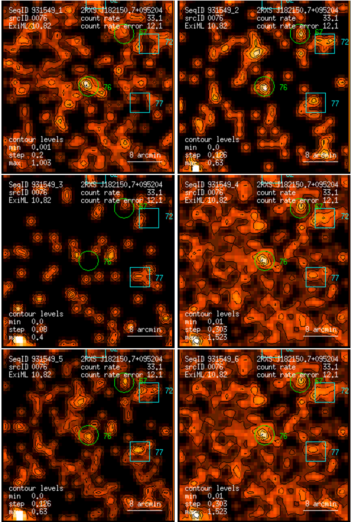
Figure 76: RASS 931549: detection 0076: band rate images, Gaussian filter: (1) PSPC channels 11 – 41, (2) 52 – 90, (3) 91 – 201, (4) 11 – 235, (5) 52 – 201, (6) 11 – 201. Broad band rates in counts/ks. Band rate contour levels in counts/ks/arcmin 2 .
