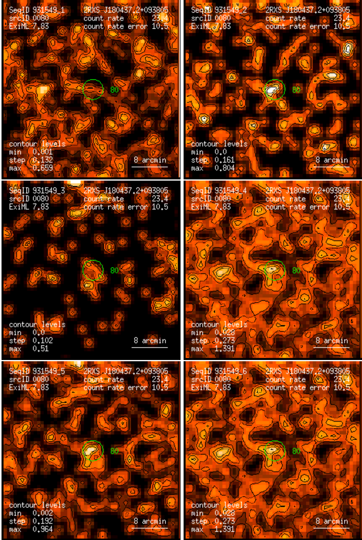
Figure 80: RASS 931549: detection 0080: band rate images, Gaussian filter: (1) PSPC channels 11 – 41, (2) 52 – 90, (3) 91 – 201, (4) 11 – 235, (5) 52 – 201, (6) 11 – 201. Broad band rates in counts/ks. Band rate contour levels in counts/ks/arcmin 2 .
