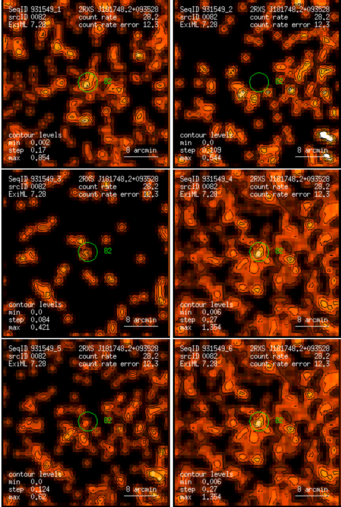
Figure 82: RASS 931549: detection 0082: band rate images, Gaussian filter: (1) PSPC channels 11 – 41, (2) 52 – 90, (3) 91 – 201, (4) 11 – 235, (5) 52 – 201, (6) 11 – 201. Broad band rates in counts/ks. Band rate contour levels in counts/ks/arcmin 2 .
