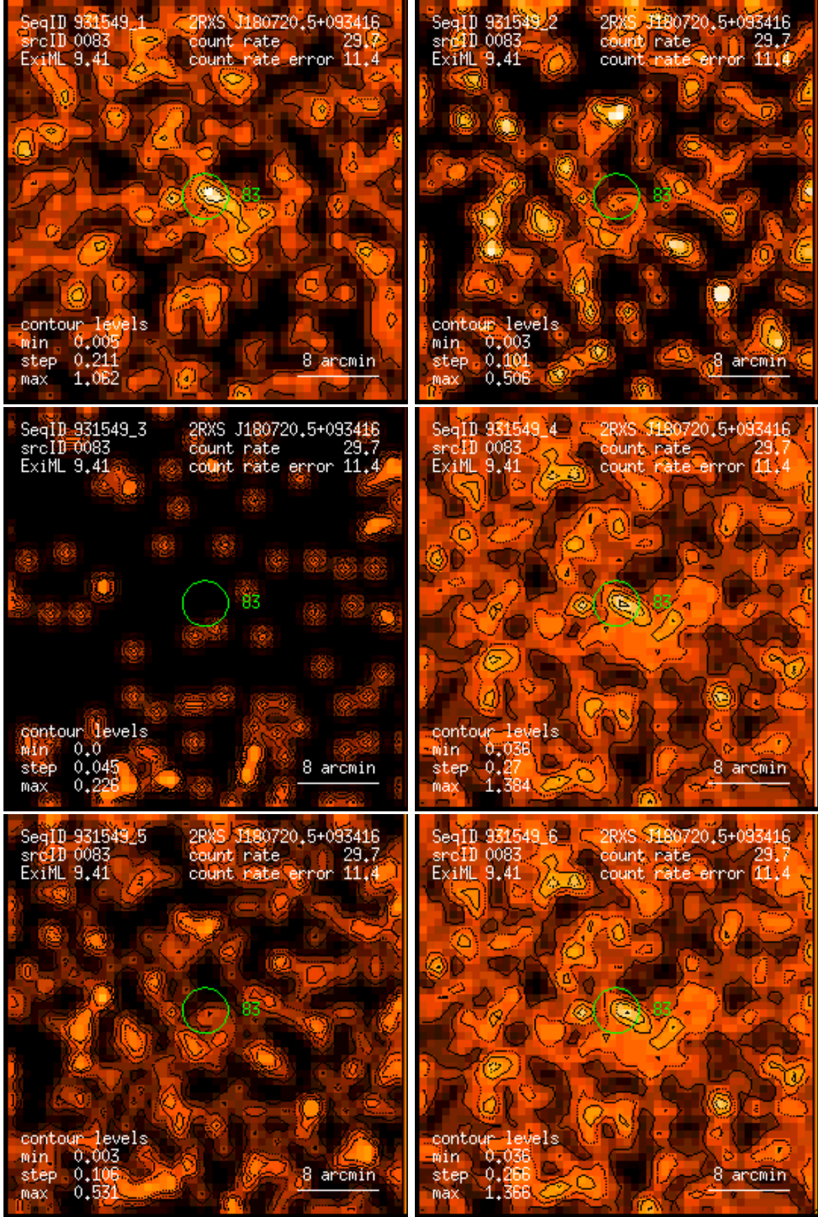
Figure 83: RASS 931549: detection 0083: band rate images, Gaussian filter: (1) PSPC channels 11 – 41, (2) 52 – 90, (3) 91 – 201, (4) 11 – 235, (5) 52 – 201, (6) 11 – 201. Broad band rates in counts/ks. Band rate contour levels in counts/ks/arcmin 2 .
