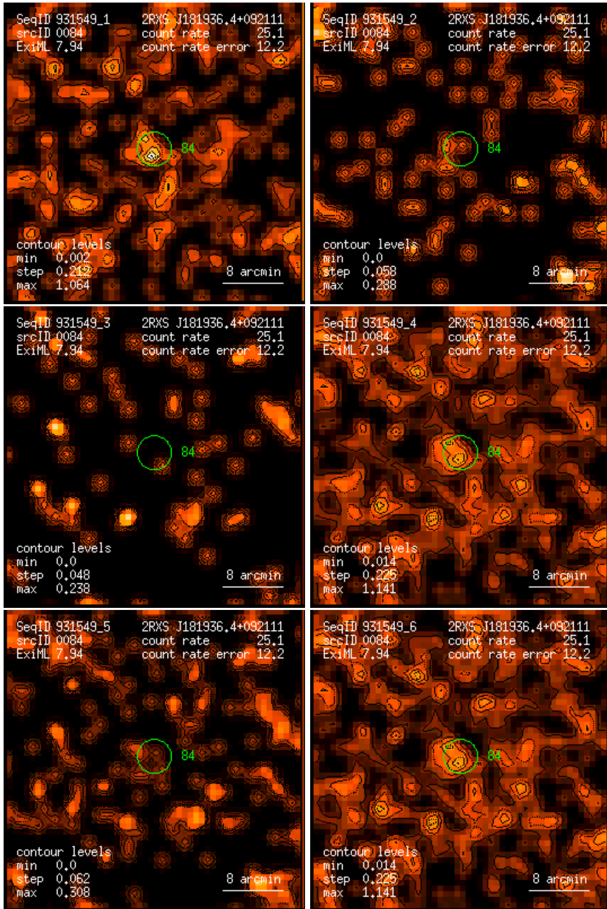
Figure 84: RASS 931549: detection 0084: band rate images, Gaussian filter: (1) PSPC channels 11 – 41, (2) 52 – 90, (3) 91 – 201, (4) 11 – 235, (5) 52 – 201, (6) 11 – 201. Broad band rates in counts/ks. Band rate contour levels in counts/ks/arcmin 2 .
