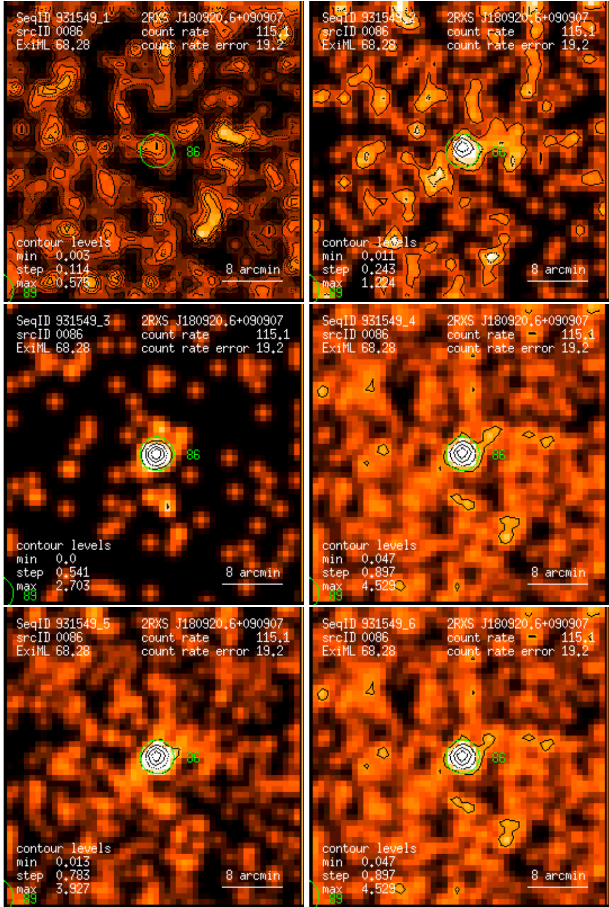
Figure 86: RASS 931549: detection 0086: band rate images, Gaussian filter: (1) PSPC channels 11 – 41, (2) 52 – 90, (3) 91 – 201, (4) 11 – 235, (5) 52 – 201, (6) 11 – 201. Broad band rates in counts/ks. Band rate contour levels in counts/ks/arcmin 2 .
