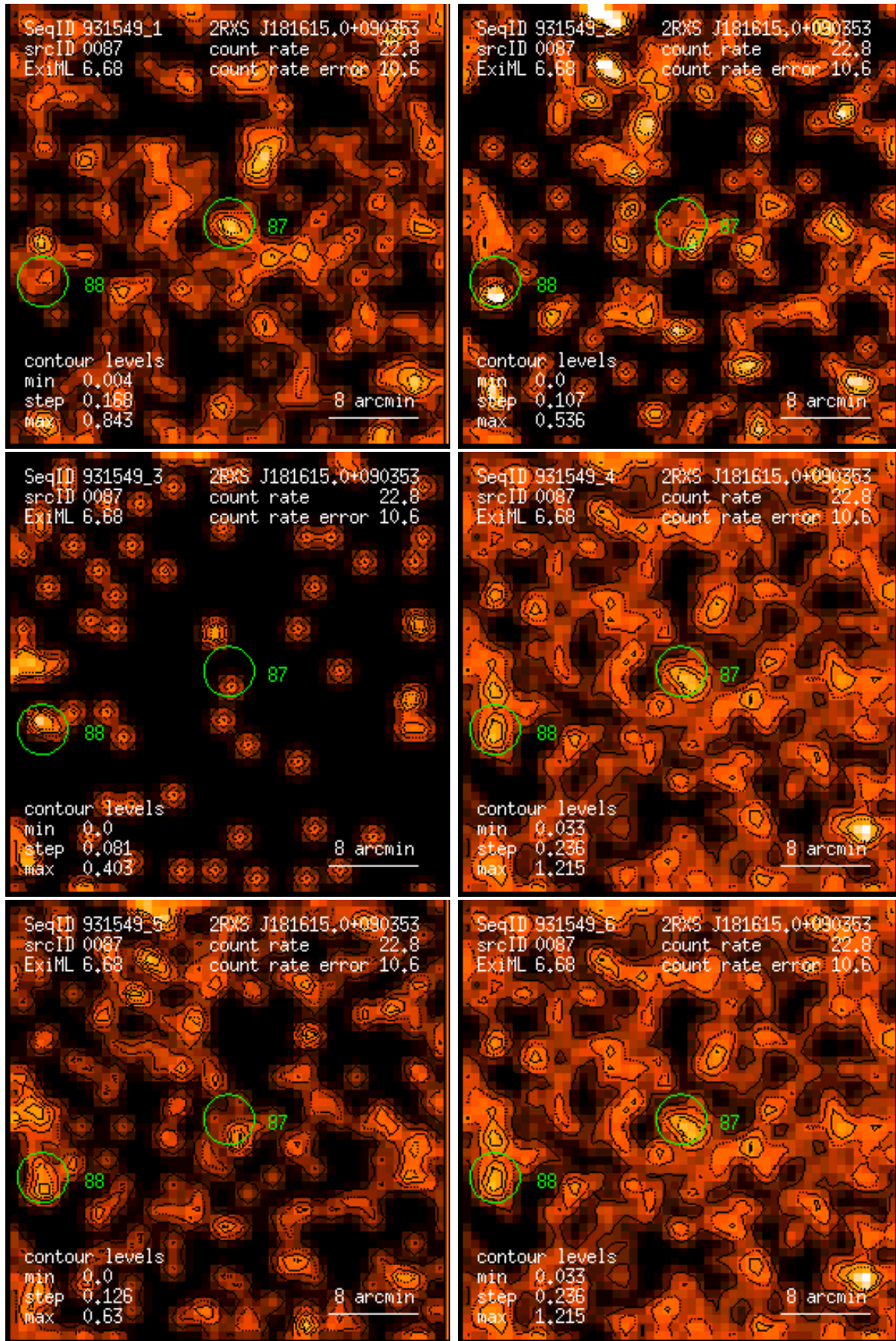
Figure 87: RASS 931549: detection 0087: band rate images, Gaussian filter: (1) PSPC channels 11 – 41, (2) 52 – 90, (3) 91 – 201, (4) 11 – 235, (5) 52 – 201, (6) 11 – 201. Broad band rates in counts/ks. Band rate contour levels in counts/ks/arcmin 2 .
