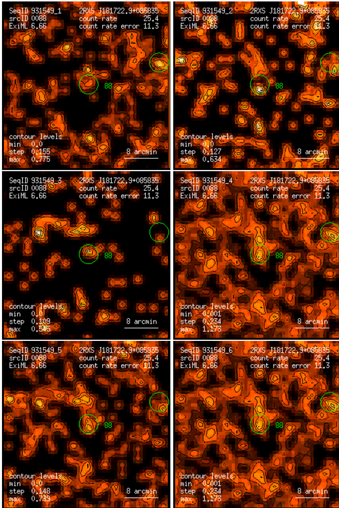
Figure 88: RASS 931549: detection 0088: band rate images, Gaussian filter: (1) PSPC channels 11 – 41, (2) 52 – 90, (3) 91 – 201, (4) 11 – 235, (5) 52 – 201, (6) 11 – 201. Broad band rates in counts/ks. Band rate contour levels in counts/ks/arcmin 2 .
