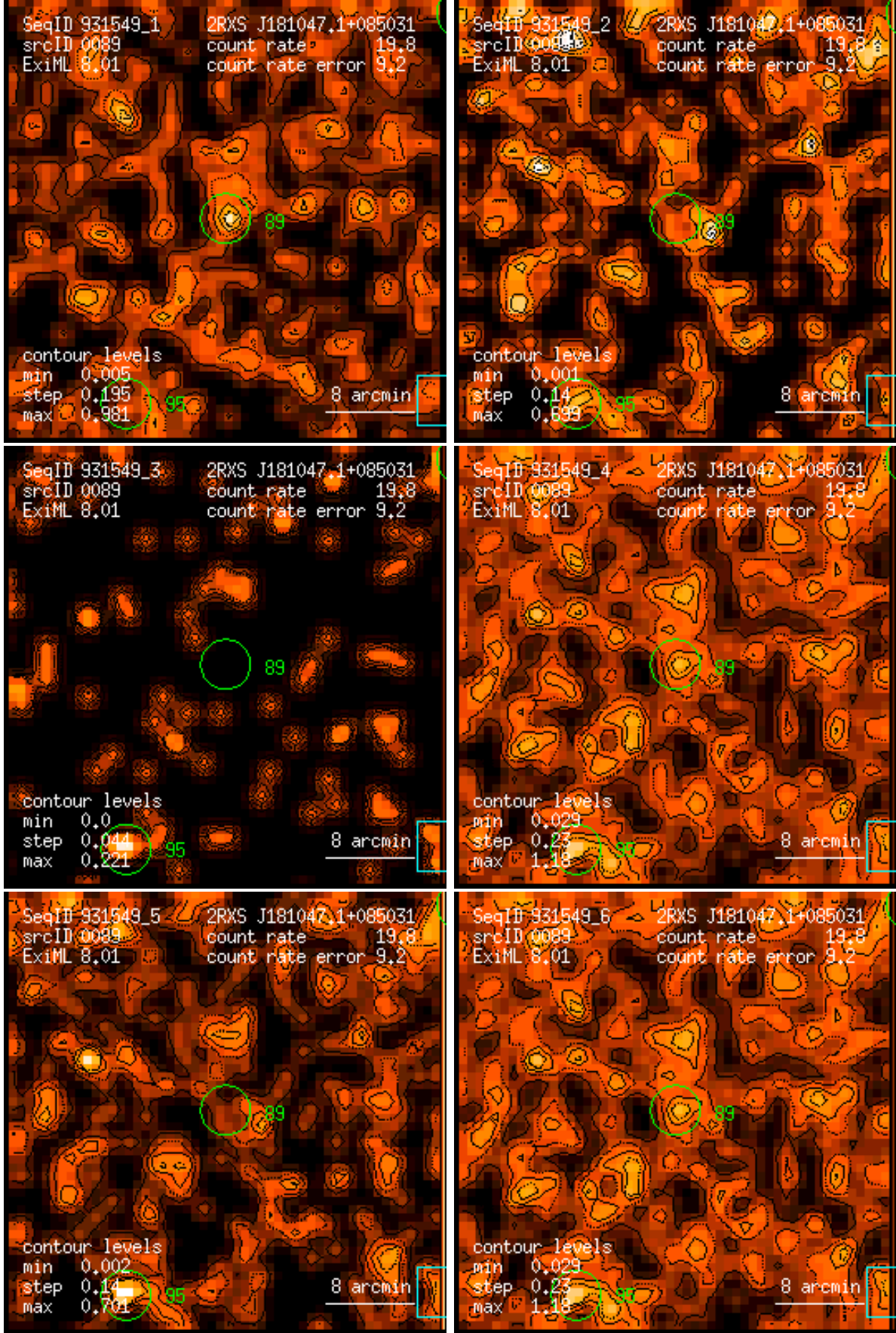
Figure 89: RASS 931549: detection 0089: band rate images, Gaussian filter: (1) PSPC channels 11 – 41, (2) 52 – 90, (3) 91 – 201, (4) 11 – 235, (5) 52 – 201, (6) 11 – 201. Broad band rates in counts/ks. Band rate contour levels in counts/ks/arcmin 2 .
