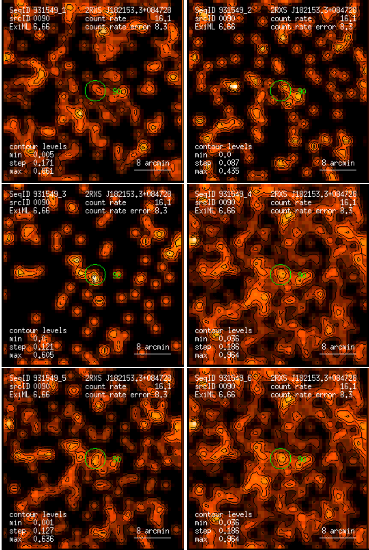
Figure 90: RASS 931549: detection 0090: band rate images, Gaussian filter: (1) PSPC channels 11 – 41, (2) 52 – 90, (3) 91 – 201, (4) 11 – 235, (5) 52 – 201, (6) 11 – 201. Broad band rates in counts/ks. Band rate contour levels in counts/ks/arcmin 2 .
