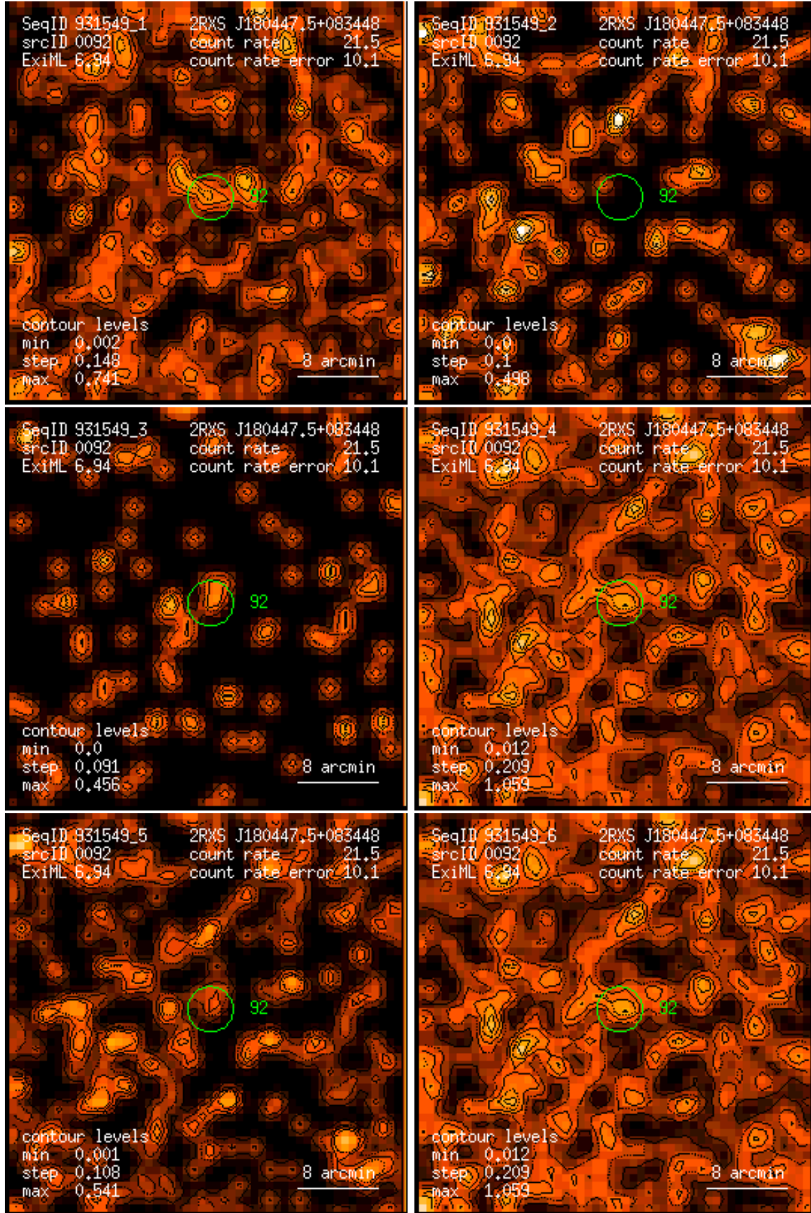
Figure 92: RASS 931549: detection 0092: band rate images, Gaussian filter: (1) PSPC channels 11 – 41, (2) 52 – 90, (3) 91 – 201, (4) 11 – 235, (5) 52 – 201, (6) 11 – 201. Broad band rates in counts/ks. Band rate contour levels in counts/ks/arcmin 2 .
