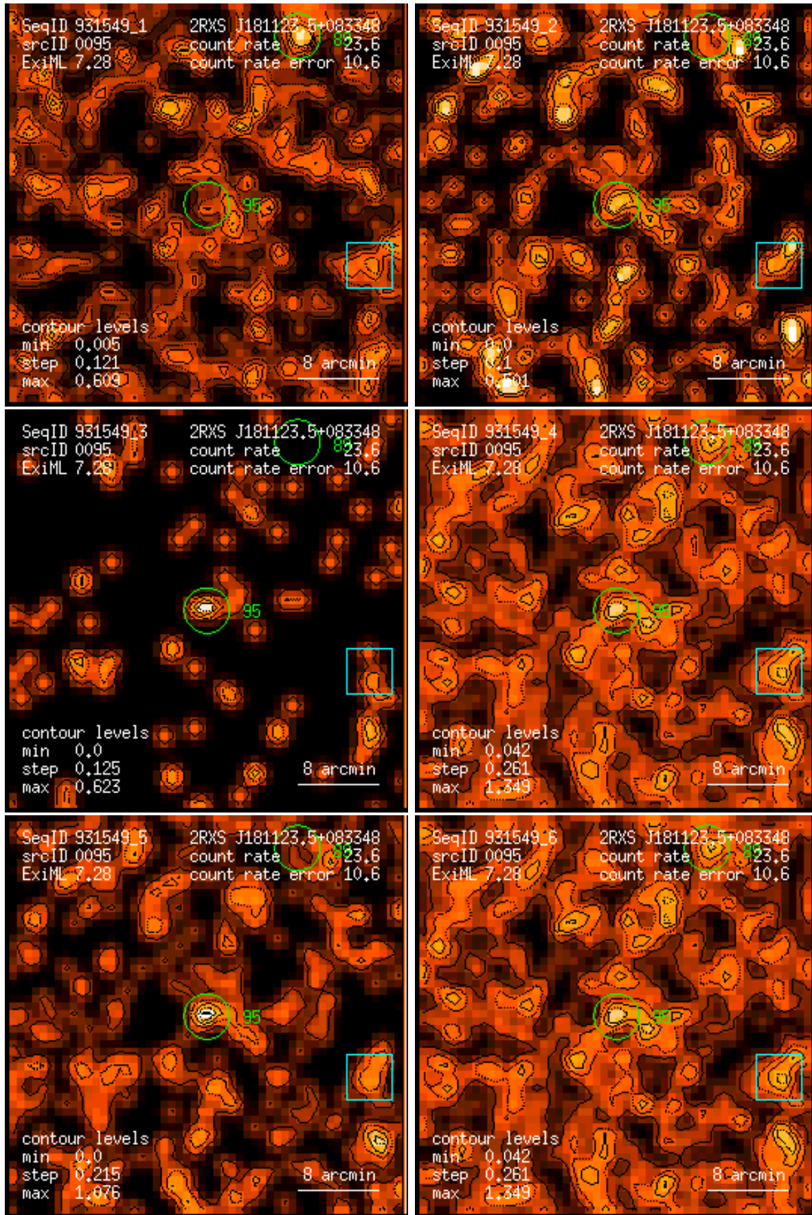
Figure 95: RASS 931549: detection 0095: band rate images, Gaussian filter: (1) PSPC channels 11 – 41, (2) 52 – 90, (3) 91 – 201, (4) 11 – 235, (5) 52 – 201, (6) 11 – 201. Broad band rates in counts/ks. Band rate contour levels in counts/ks/arcmin 2 .
