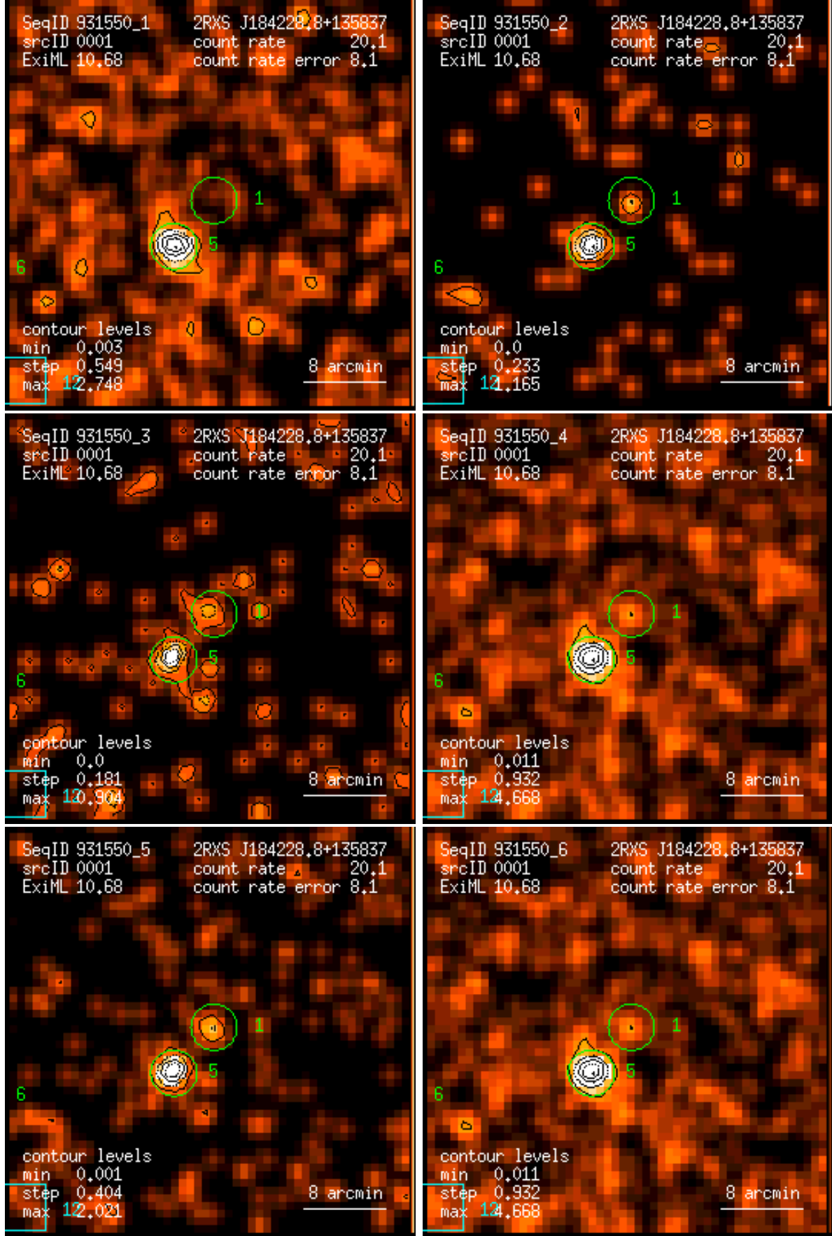
Figure 1: RASS 931550: detection 0001: band rate images, Gaussian filter: (1) PSPC channels 11 – 41, (2) 52 – 90, (3) 91 – 201, (4) 11 – 235, (5) 52 – 201, (6) 11 – 201. Broad band rates in counts/ks. Band rate contour levels in counts/ks/arcmin 2 .
