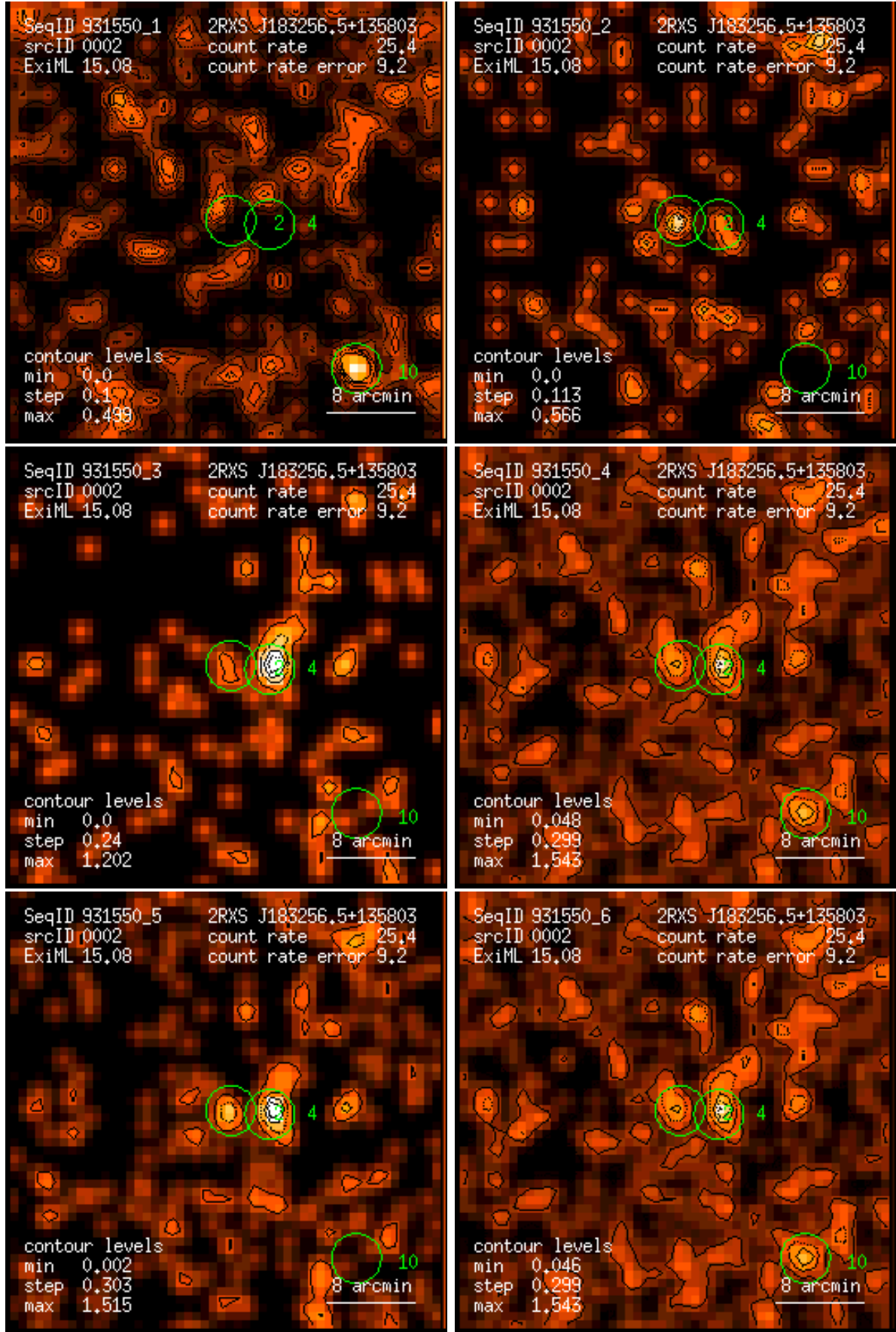
Figure 2: RASS 931550: detection 0002: band rate images, Gaussian filter: (1) PSPC channels 11 – 41, (2) 52 – 90, (3) 91 – 201, (4) 11 – 235, (5) 52 – 201, (6) 11 – 201. Broad band rates in counts/ks. Band rate contour levels in counts/ks/arcmin 2 .
