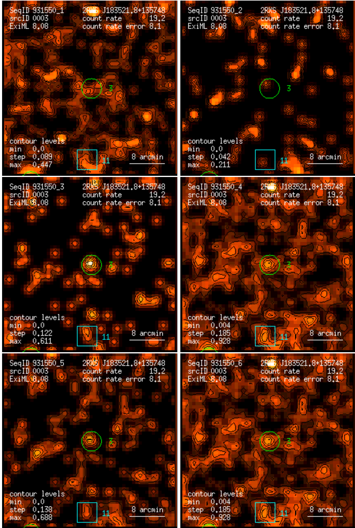
Figure 3: RASS 931550: detection 0003: band rate images, Gaussian filter: (1) PSPC channels 11 – 41, (2) 52 – 90, (3) 91 – 201, (4) 11 – 235, (5) 52 – 201, (6) 11 – 201. Broad band rates in counts/ks. Band rate contour levels in counts/ks/arcmin 2 .
