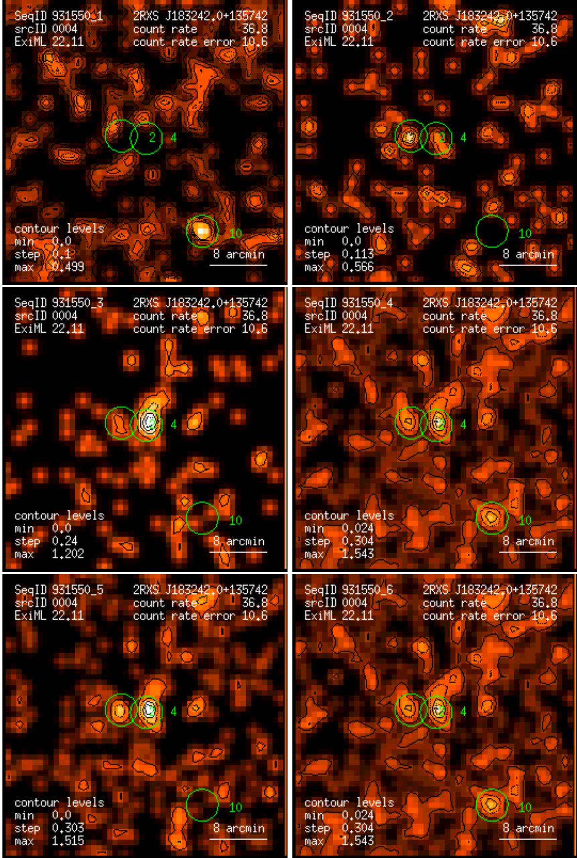
Figure 4: RASS 931550: detection 0004: band rate images, Gaussian filter: (1) PSPC channels 11 – 41, (2) 52 – 90, (3) 91 – 201, (4) 11 – 235, (5) 52 – 201, (6) 11 – 201. Broad band rates in counts/ks. Band rate contour levels in counts/ks/arcmin 2 .
