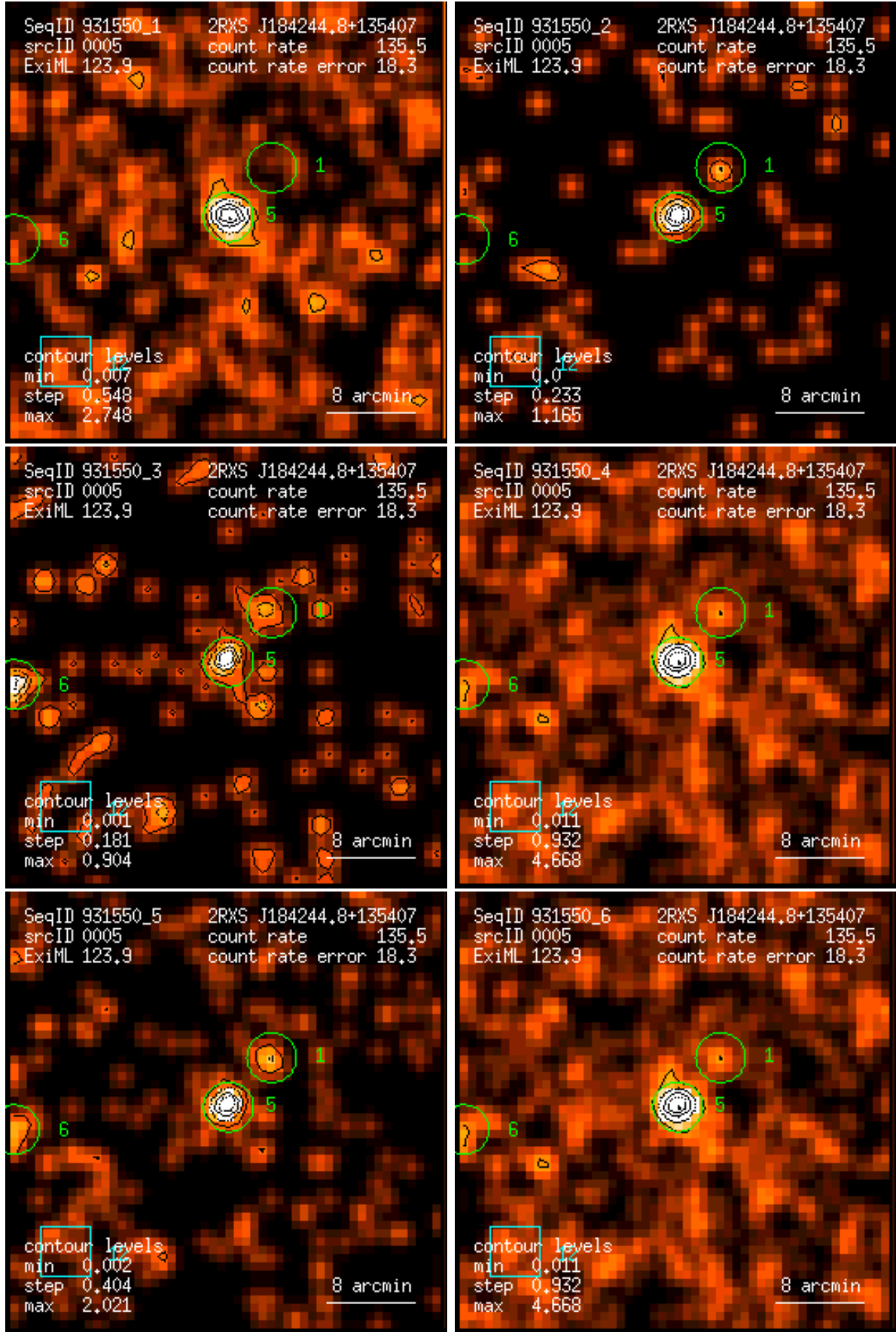
Figure 5: RASS 931550: detection 0005: band rate images, Gaussian filter: (1) PSPC channels 11 – 41, (2) 52 – 90, (3) 91 – 201, (4) 11 – 235, (5) 52 – 201, (6) 11 – 201. Broad band rates in counts/ks. Band rate contour levels in counts/ks/arcmin 2 .
