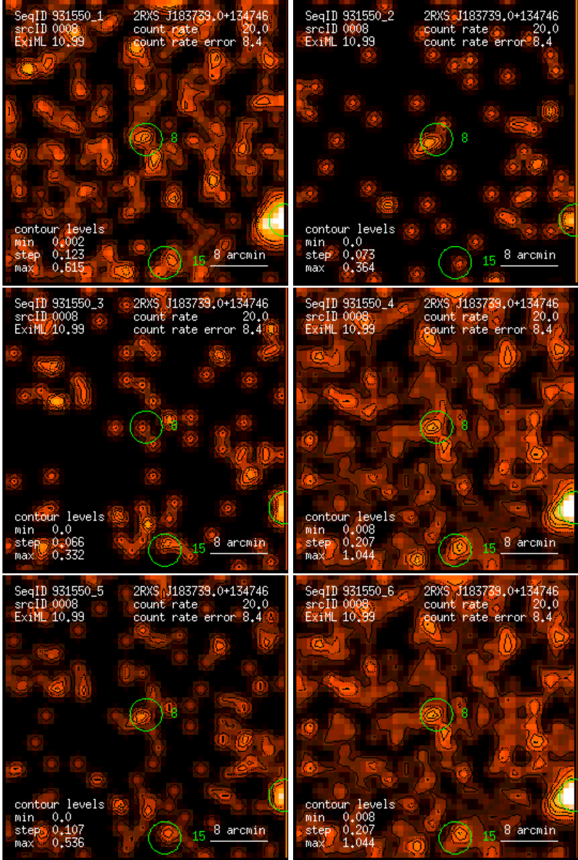
Figure 8: RASS 931550: detection 0008: band rate images, Gaussian filter: (1) PSPC channels 11 – 41, (2) 52 – 90, (3) 91 – 201, (4) 11 – 235, (5) 52 – 201, (6) 11 – 201. Broad band rates in counts/ks. Band rate contour levels in counts/ks/arcmin 2 .
