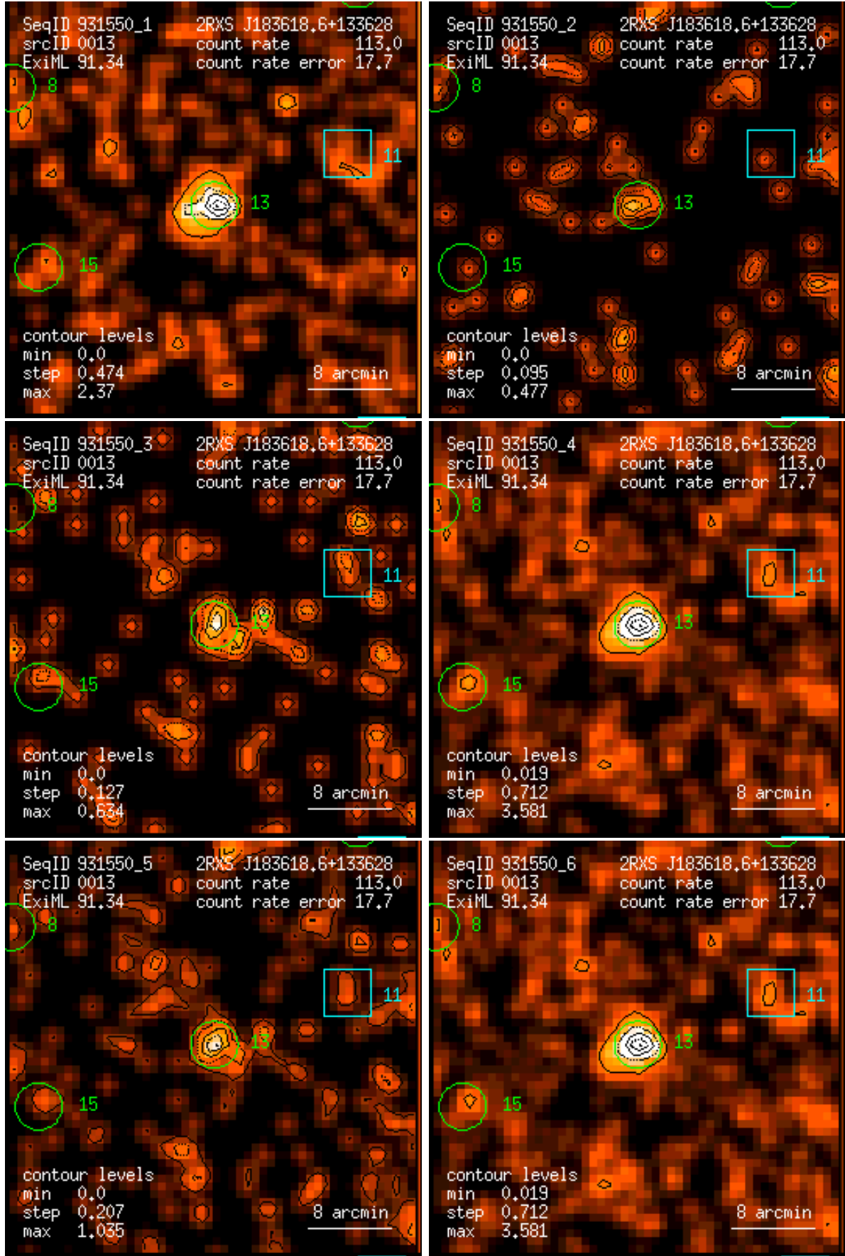
Figure 13: RASS 931550: detection 0013: band rate images, Gaussian filter: (1) PSPC channels 11 – 41, (2) 52 – 90, (3) 91 – 201, (4) 11 – 235, (5) 52 – 201, (6) 11 – 201. Broad band rates in counts/ks. Band rate contour levels in counts/ks/arcmin 2 .
