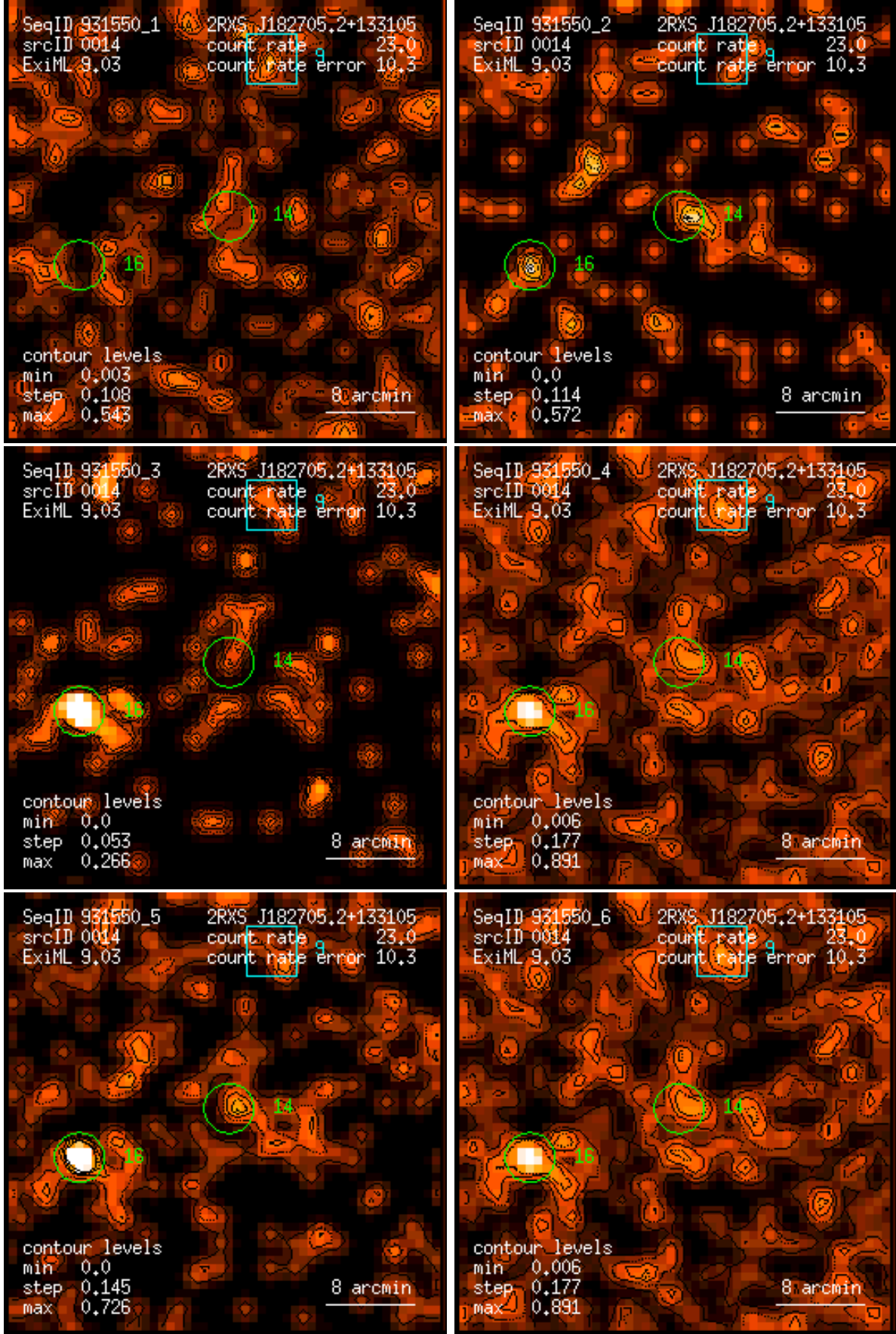
Figure 14: RASS 931550: detection 0014: band rate images, Gaussian filter: (1) PSPC channels 11 – 41, (2) 52 – 90, (3) 91 – 201, (4) 11 – 235, (5) 52 – 201, (6) 11 – 201. Broad band rates in counts/ks. Band rate contour levels in counts/ks/arcmin 2 .
