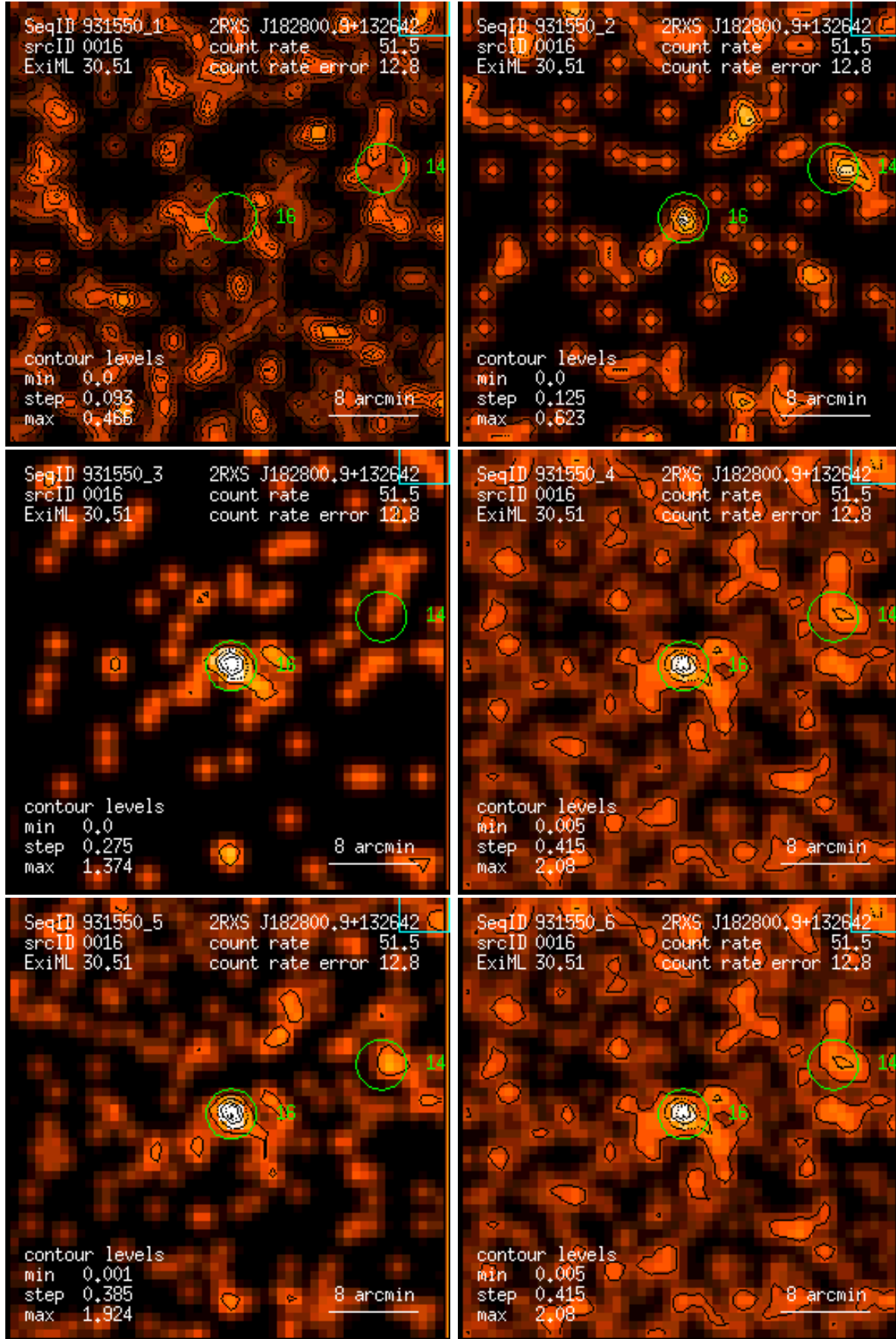
Figure 16: RASS 931550: detection 0016: band rate images, Gaussian filter: (1) PSPC channels 11 – 41, (2) 52 – 90, (3) 91 – 201, (4) 11 – 235, (5) 52 – 201, (6) 11 – 201. Broad band rates in counts/ks. Band rate contour levels in counts/ks/arcmin 2 .
