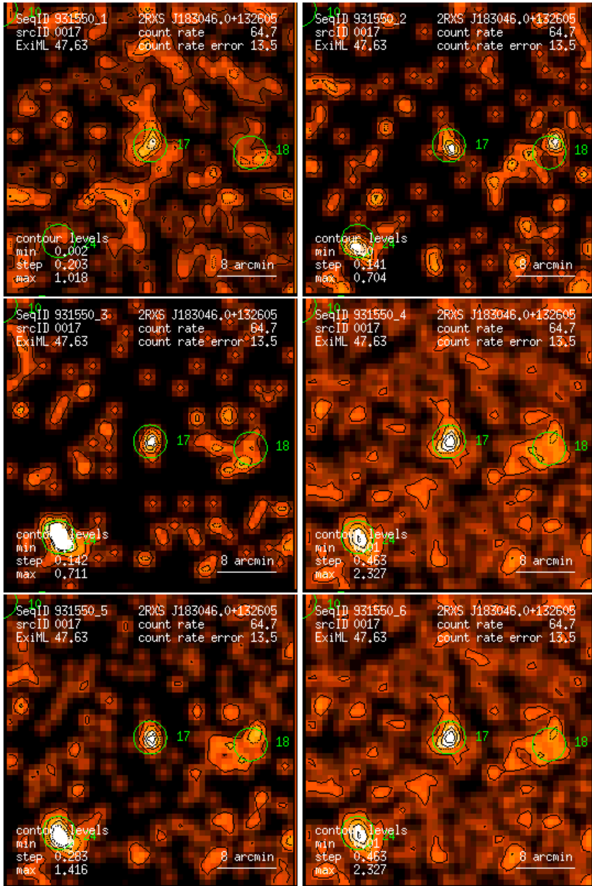
Figure 17: RASS 931550: detection 0017: band rate images, Gaussian filter: (1) PSPC channels 11 – 41, (2) 52 – 90, (3) 91 – 201, (4) 11 – 235, (5) 52 – 201, (6) 11 – 201. Broad band rates in counts/ks. Band rate contour levels in counts/ks/arcmin 2 .
