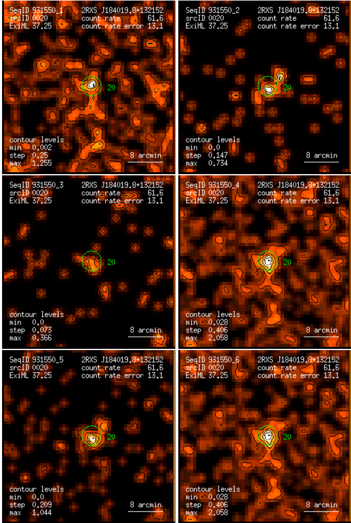
Figure 20: RASS 931550: detection 0020: band rate images, Gaussian filter: (1) PSPC channels 11 – 41, (2) 52 – 90, (3) 91 – 201, (4) 11 – 235, (5) 52 – 201, (6) 11 – 201. Broad band rates in counts/ks. Band rate contour levels in counts/ks/arcmin 2 .
