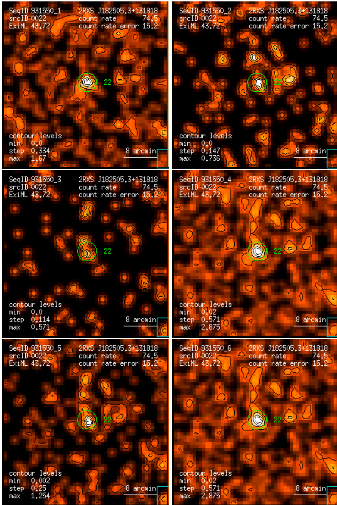
Figure 22: RASS 931550: detection 0022: band rate images, Gaussian filter: (1) PSPC channels 11 – 41, (2) 52 – 90, (3) 91 – 201, (4) 11 – 235, (5) 52 – 201, (6) 11 – 201. Broad band rates in counts/ks. Band rate contour levels in counts/ks/arcmin 2 .
