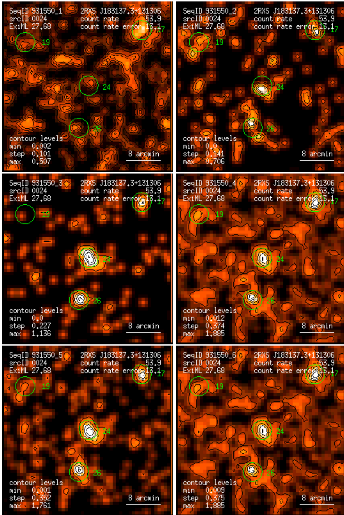
Figure 24: RASS 931550: detection 0024: band rate images, Gaussian filter: (1) PSPC channels 11 – 41, (2) 52 – 90, (3) 91 – 201, (4) 11 – 235, (5) 52 – 201, (6) 11 – 201. Broad band rates in counts/ks. Band rate contour levels in counts/ks/arcmin 2 .
