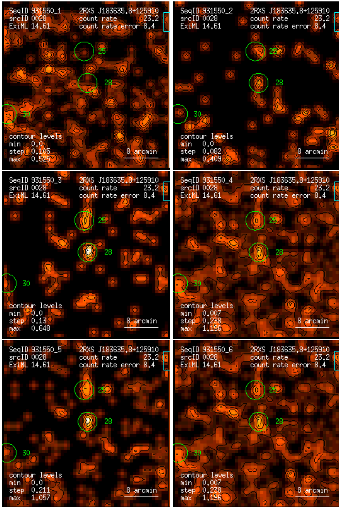
Figure 28: RASS 931550: detection 0028: band rate images, Gaussian filter: (1) PSPC channels 11 – 41, (2) 52 – 90, (3) 91 – 201, (4) 11 – 235, (5) 52 – 201, (6) 11 – 201. Broad band rates in counts/ks. Band rate contour levels in counts/ks/arcmin 2 .
