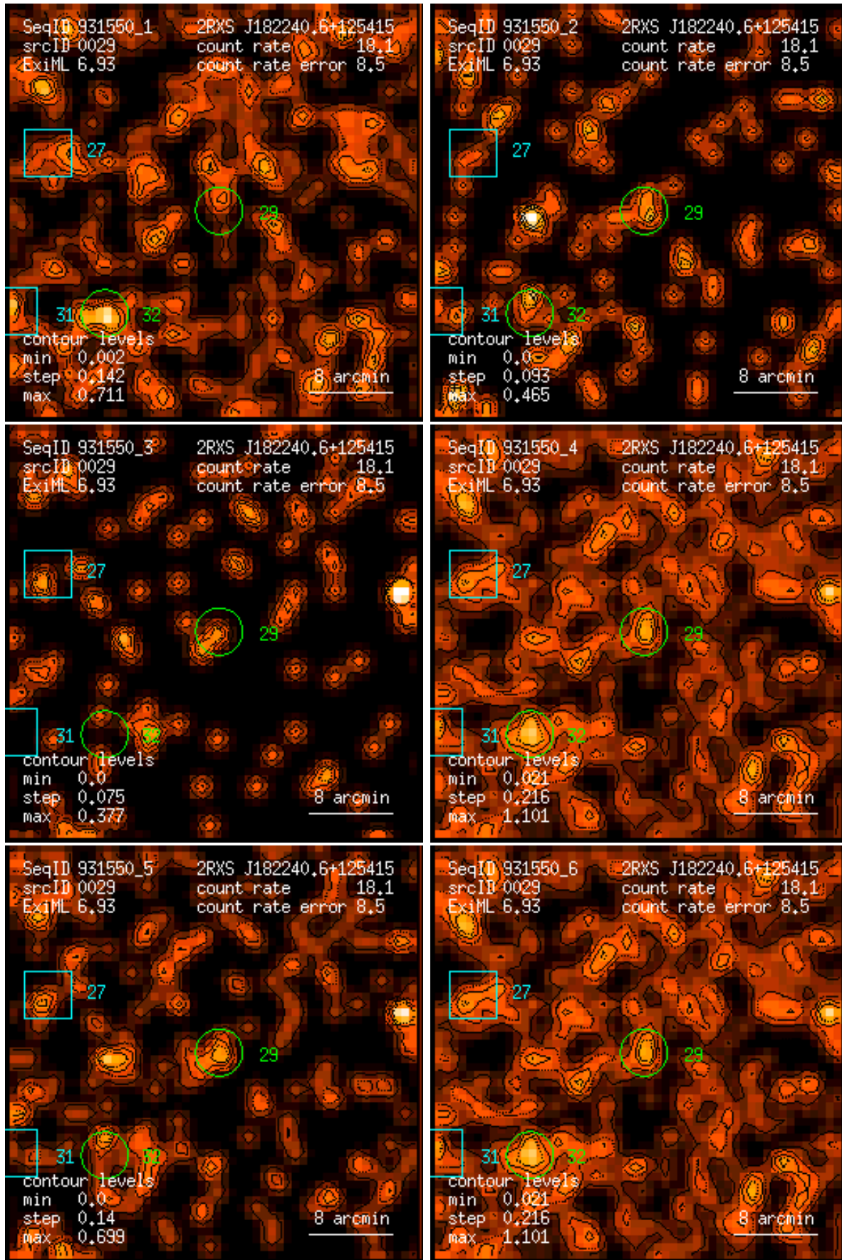
Figure 29: RASS 931550: detection 0029: band rate images, Gaussian filter: (1) PSPC channels 11 – 41, (2) 52 – 90, (3) 91 – 201, (4) 11 – 235, (5) 52 – 201, (6) 11 – 201. Broad band rates in counts/ks. Band rate contour levels in counts/ks/arcmin 2 .
