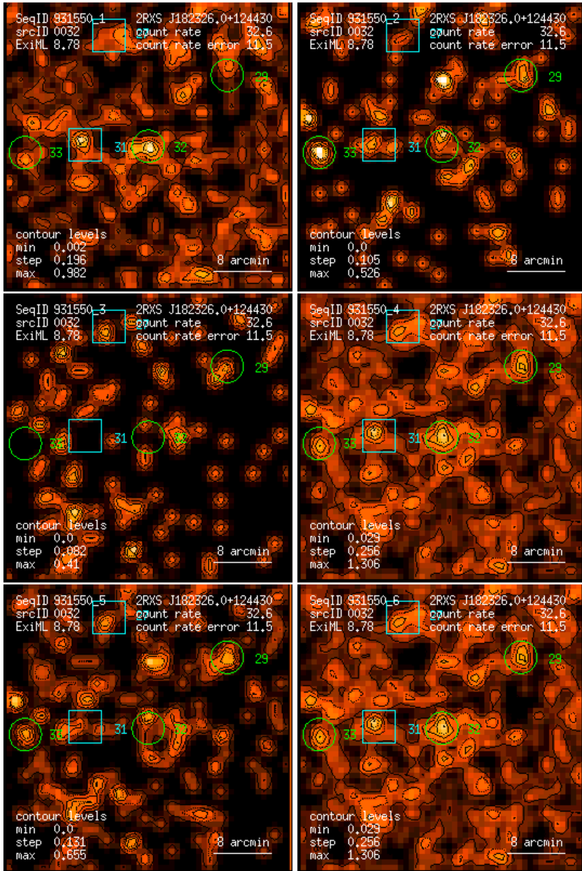
Figure 32: RASS 931550: detection 0032: band rate images, Gaussian filter: (1) PSPC channels 11 – 41, (2) 52 – 90, (3) 91 – 201, (4) 11 – 235, (5) 52 – 201, (6) 11 – 201. Broad band rates in counts/ks. Band rate contour levels in counts/ks/arcmin 2 .
