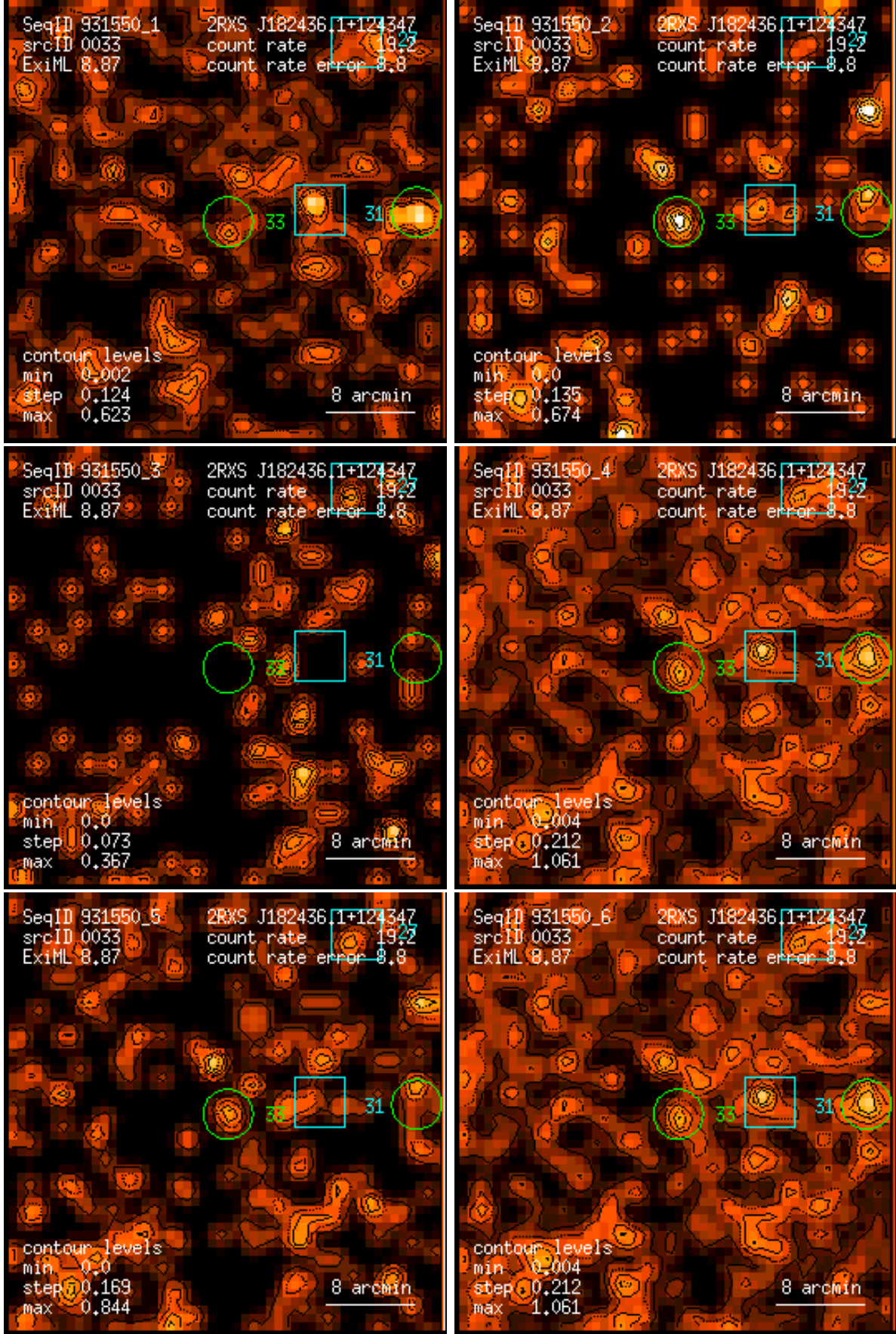
Figure 33: RASS 931550: detection 0033: band rate images, Gaussian filter: (1) PSPC channels 11 – 41, (2) 52 – 90, (3) 91 – 201, (4) 11 – 235, (5) 52 – 201, (6) 11 – 201. Broad band rates in counts/ks. Band rate contour levels in counts/ks/arcmin 2 .
